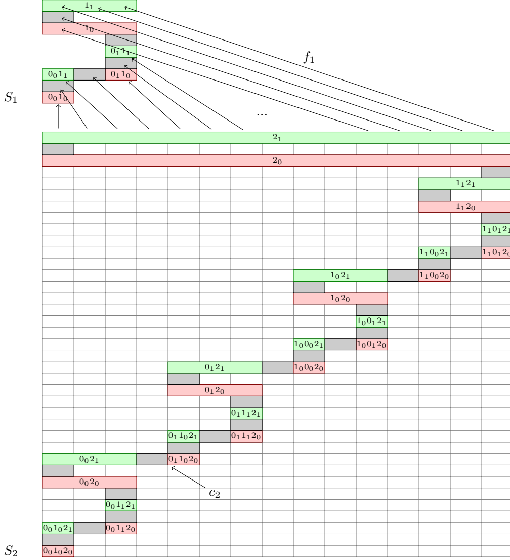
FIGURE 2. The embedding f_1 : B_2 \hookrightarrow S_1 .
