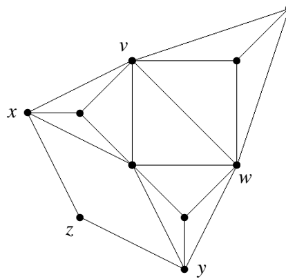
Figure 3.1. This graph is rigid so has exactly one rigid component. There are three redundantly rigid components, consisting of the union of the three copies of K_4 , and the remaining two copies of K_2 . There are five M-connected components: each of the three copies of K_4 , and the remaining two copies of K_2 .
