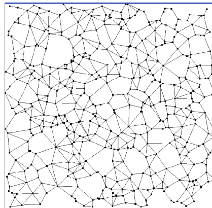
FIG. 1. The relative neighborhood graph (left) and Gabriel graph (right) on different realizations of 500 random points.
