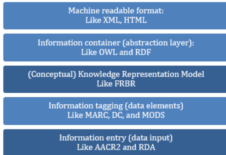
Figure 12 Linked Data Stack, Conceptual Information for Information Retrieval and Librarian Use Included
