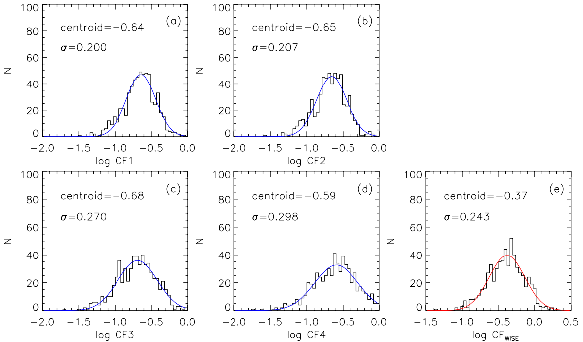
Figure 2. Distributions of MIR covering factors: CF_{MIR} = L_{MIR}/L_{bol} using the basic sample. The solid line is the Gaussian fit to the distribution; the centroid and \sigma of the Gaussian are shown in the upper left corner. Panels (a)–(d) show CF_{MIR} distributions at each band, and panel (e) shows the distribution of CF_{WISE} = L_{WISE}/L_{bol} . (A color version of this figure is available in the online journal.)
