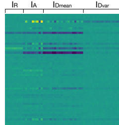
Fig. 5: Mediator Weights.
