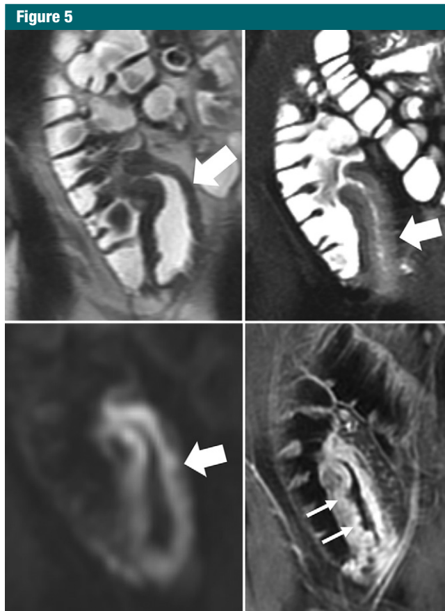
Figure 5: Imaging findings of severe inflammation of the terminal ileum at MRE, as indicated by marked wall thickening ( top left, arrow ), intramural edema or hyperintensity on a T2-weighted image with fat saturation ( top right, arrow ), increased intramural signal on high b-value diffusion-weighted images ( bottom left, arrow ), and small ulcerations on gadolinium-enhanced images ( bottom right, small white arrows ).
