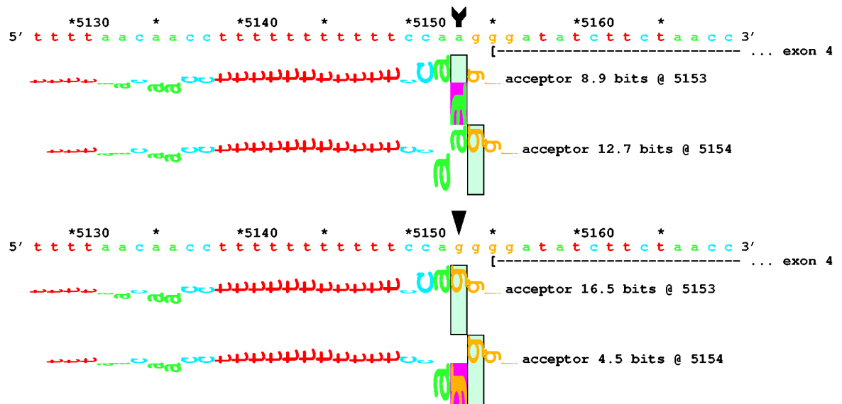
Figure 2. Sequence walkers (Schneider, 1997b) for a human acceptor site in the iduronidase synthetase gene and a mutation (indicated by an arrow). On the top sequence, the normal end of exon 4 is shown by a bracket and dashed line. The vertical rectangle on a sequence walker is the 'zero base' used to identify the location of the walker. The vertical rectangles also indicate a scale from -3 to +2 bits. A 12.7 bit acceptor at 5154 directs splicing to the correct location. Source: Adapted from (Rogan et al. , 1998).
