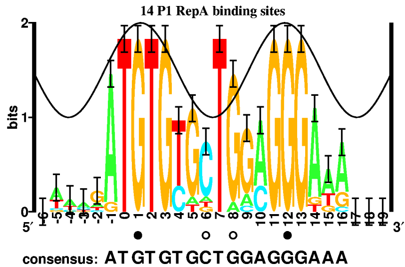
Figure 5. Sequence logo for RepA binding sites. Error bars indicate standard deviations of the entire stack height. Source: Adapted from (Schneider, 2001).
