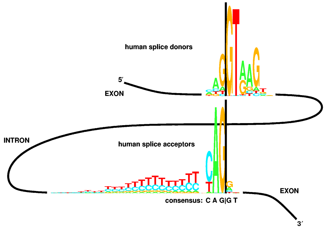
Figure 1. Sequence logos (Schneider & Stephens, 1990) for human donor and acceptor splice junctions (Stephens & Schneider, 1992) compared to the consensus sequence for both sites. Source: Adapted from (Stephens & Schneider, 1992).
