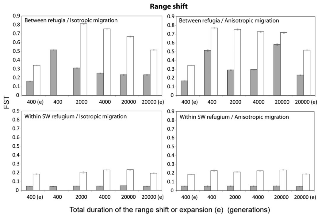
Fig. 6. Average F_{ST} observed in refuge areas after range shifts occurring at different speeds. Upper graphs: F_{ST} values observed between SW and SE refuges. Lower graphs: F_{ST} values observed between samples within SW refugium, SE refugium produced similar results (not showed) to the SW refugium. (e) indicates cases where there has been no range shift after the initial range expansion. Bar colors represent results obtained for different migration rates: gray, m_1 = 0.05 ; white, m_1 = 0.01 . The left graphs correspond to scenarios simulated with isotropic migration at rate, whereas right graphs correspond to scenarios simulated under anisotropic migration ( m_2 = 0.20 , m_3 = 0.01 ). Note that no data are available when the range shift lasts only 400 generations in case of isotropic migration and a small migration rate m_1 = 0.01 due to population extinction (see text). Error bars indicate 1.96 \times standard error intervals obtained from our 1,000 simulations.
