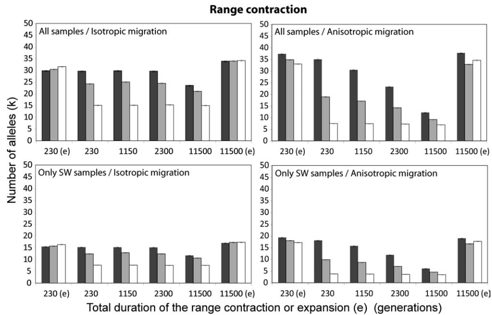
FIG. 3. Average number of alleles ( k ) observed in refuge areas after range contractions of different speeds. Upper graphs: Total number of alleles observed among all pooled samples. Lower graphs: Number of alleles observed among the samples of the SW refugium (results for SE refugium are similar but not shown). (e) indicates cases where there has been no range contraction after the initial range expansion. Bar colors represent results obtained for different refugial isolation times: black, 10 generations; gray, 100 generations; white, 1,000 generations. The left graphs correspond to scenarios simulated with isotropic migration at rate m_1 = 0.05 , whereas right graphs correspond to scenarios simulated under anisotropic migration ( m_1 = 0.05 , m_2 = 0.20 , m_3 = 0.01 ). Error bars indicate 1.96 \times standard error intervals obtained from our 1,000 simulations.
