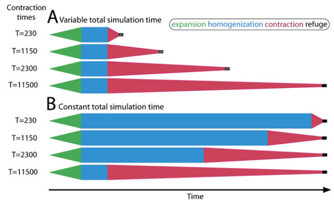
FIG. 2. Schematic representation of the main types of range contractions that were simulated. In each case, after an initial phase of range expansion (green), the species range remains constant (blue) for some time allowing for the homogenization of genetic diversity among populations. Then, a phase of range contraction occurs (red), which is followed by a final phase of evolution in refuge areas (black). Genetic diversity is sampled at the end of the four phases. We also distinguish scenarios where the total simulation time varies according to the duration of the range contraction (A) and scenarios where the total simulation time is constant despite variable contraction times that are compensated by a proportional change in the homogenization time (B). Note that other scenarios allowing for variable evolution times in refuge areas are not shown here but would be represented by variable lengths of the black bar.
