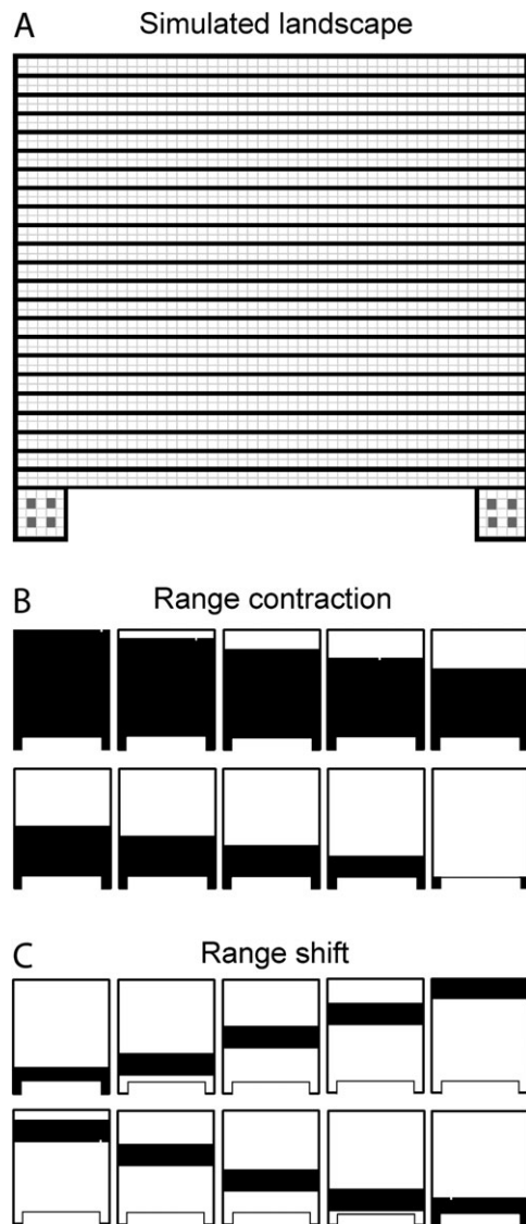
Fig. 1. Simulated landscape and spatial processes. (A) The simulation landscape consists in a 2D lattice made up of 51 \times 51 demes. The lattice is virtually divided into 23 horizontal layers of 2 \times 51 demes, plus a 5-deme thick layer containing two refugia areas of size 5 \times 5 demes. The four gray dots in each refugia represent the sampled demes. In panes B and C, black areas represent demes occupied at different times of the three different spatial processes, and white areas are empty. The timelines runs from left to right on both lines of panes B and C. The range contractions and range shifts shown in panes B and C, respectively, follow a range expansion after a homogenization time (see text and fig. 2). This range expansion always starts in the middle of the left refugia area. Note that range contractions and range shifts can proceed at different speeds as described in figure 2.
