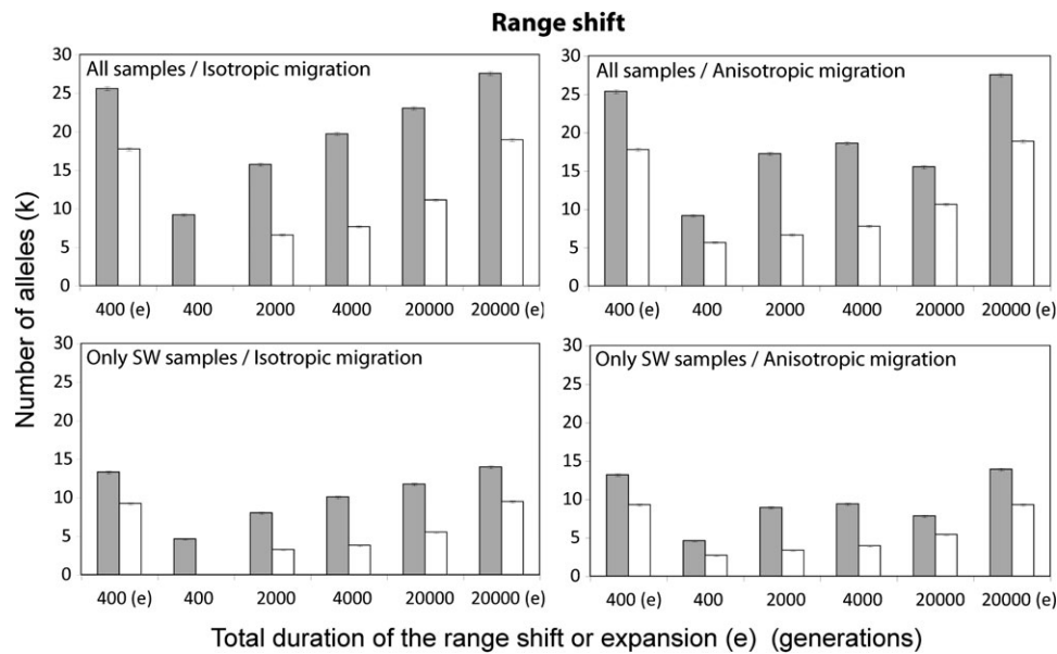
FIG. 5. Average number of alleles observed in refuge areas after range shifts occurring at different speeds. Upper graphs: Total number of alleles observed among all pooled samples. Lower graphs: Number of different alleles observed among the samples of the SW refugium (results for the SE refugium are similar but not shown). ( e ) indicates cases where there has been no range shift after the initial range expansion. Bar colors represent results obtained for different migration rates: gray, m_1 = 0.05 ; white, m_1 = 0.01 . The left graphs correspond to scenarios simulated with isotropic migration, whereas right graphs correspond to scenarios simulated under anisotropic migration ( m_2 = 0.20 , m_3 = 0.01 ). Note that no data are available when the range shift lasts only 400 generations in case of isotropic migration and a small migration rate m_1 = 0.01 due to population extinction (see text). Error bars indicate 1.96 \times standard error intervals obtained from our 1,000 simulations.
