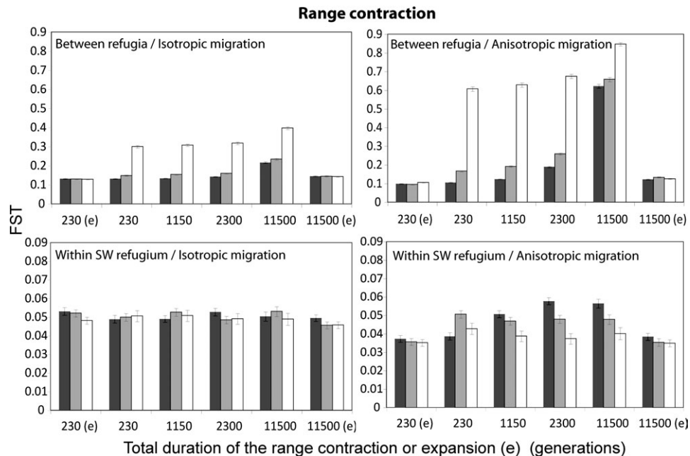
FIG. 4. Average F_{ST} observed in refuge areas after a range contraction of different speeds. Upper graphs: F_{ST} values observed between SW and SE refuges. Lower graphs: F_{ST} values observed between samples within SW refugium (results for the SE refugium are similar but not shown). Note the zoomed y-axis on the lower graphs. (e) indicates cases where there has been no range contraction after the initial range expansion. Bar colors represent results obtained for different refugial isolation times: black, 10 generations; gray, 100 generations; white, 1,000 generations. The left graphs correspond to scenarios simulated with isotropic migration at rate m_1 = 0.05 , whereas right graphs correspond to scenarios simulated under anisotropic migration ( m_1 = 0.05 , m_2 = 0.20 , m_3 = 0.01 ). Error bars indicate 1.96 \times standard error intervals obtained from our 1,000 simulations.
