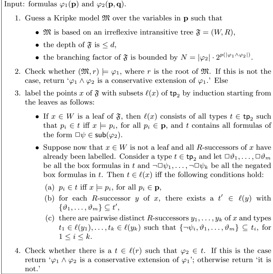
Figure 1. Deciding non-conservativeness for \mathbf{K} .
