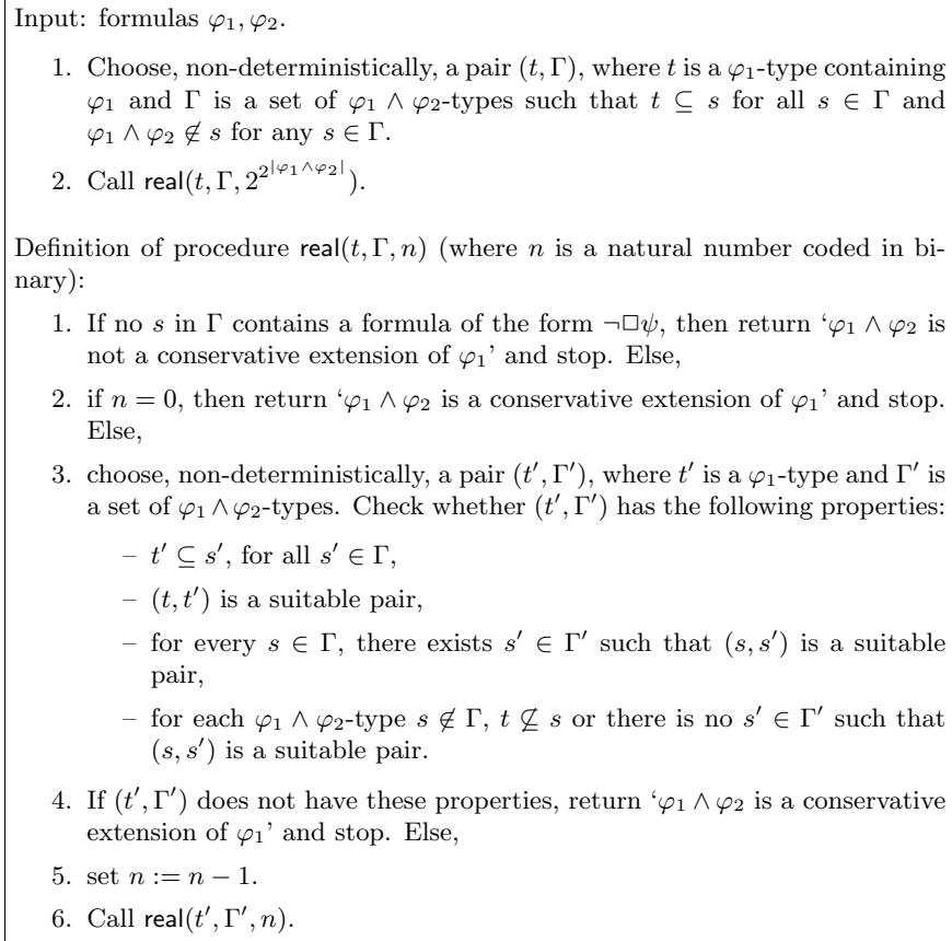
Figure 4. Deciding non-conservativeness for GL.3 .
