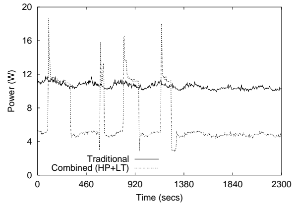
Figure 7: Power consumption of traditional and Combined systems for the Clarknet trace. Peaks of 50% utilization.
