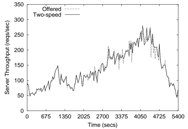
Figure 14: Server throughput for the proxy trace with the two-speed disk. Peaks of 80% utilization.
