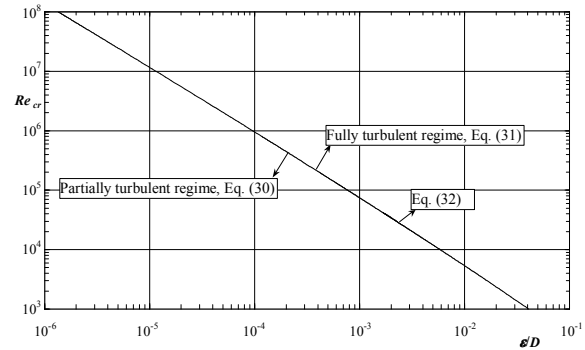
Figure 2. The critical Reynolds number Re_{cr} and the relative roughness.
