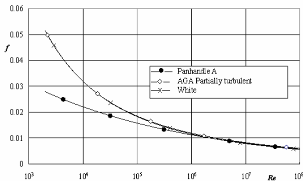
Figure 3 Comparison of attrition factors for Panhandle A, AGA p/t and White equations.
