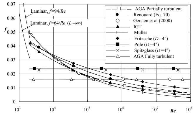
Figure 5 Evolution of friction factors used in several, previously discussed, flow equations.
