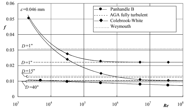
Figure 4 Friction coefficients used in the Panhandle B, AGA fully turbulent, Colebrook-White and Weymouth.
