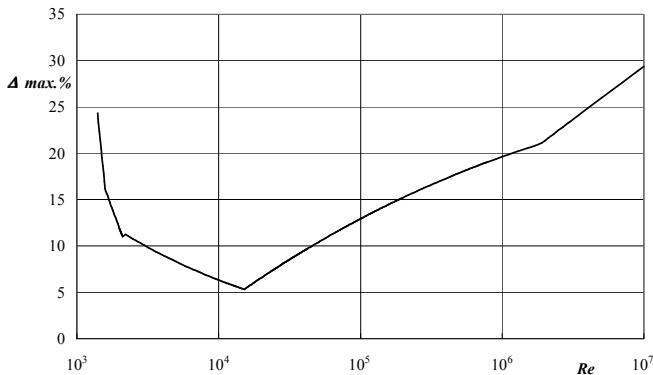
Figure 6 Maximum variation of the friction factor relatively to its average value when calculated through the following equations: AGA p/t, Renouard, Muller, IGT and for laminar flow regime.
