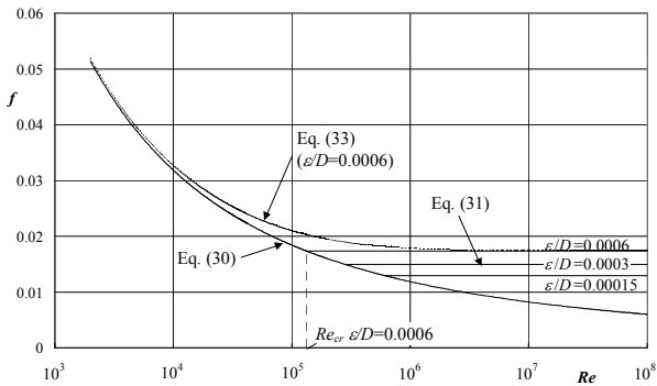
Figure 1. Influence of the relative roughness in the regime transition from hydraulically smooth to rough pipes turbulent flow.
