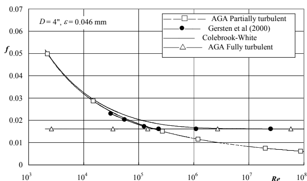
Figure 7 Comparison among AGA, Colebrook-White and Gersten et al equations (2000).
