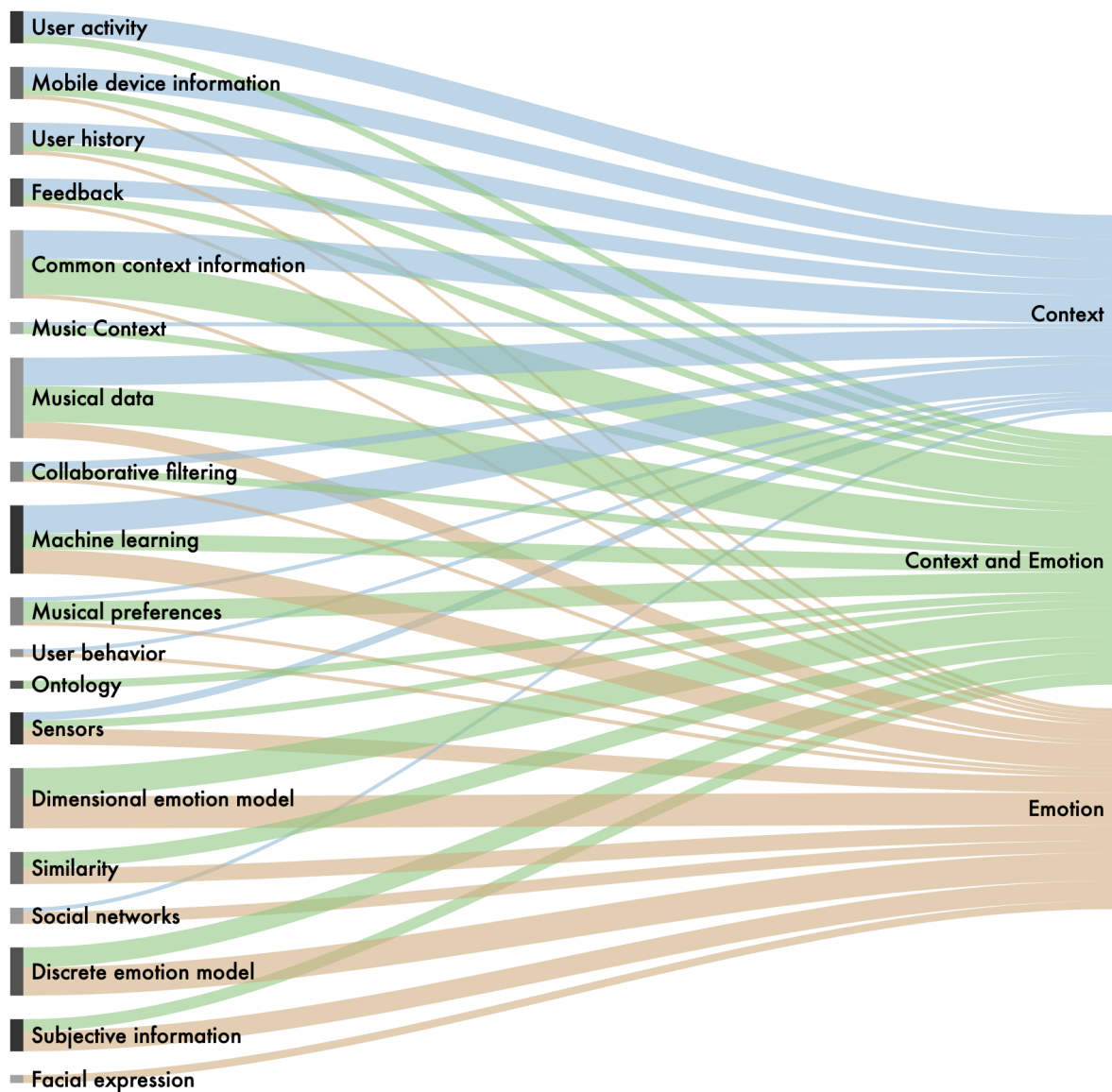
Fig. 5: Correlation between music recommendation approaches.
