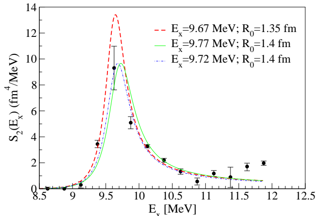
FIG. 4: (Color online) The spin 2 strength function ( S_2(E_x) ) extracted from the multipole decomposition analysis [17] (data points) compared with the R-matrix line-shapes (equation 1) associated with different channel radii and excitation energies.
