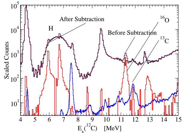
FIG. 2: (Color online) Analysis of background contributions to the ^{12}\text{C} excitation energy spectrum populated in \alpha -inelastic scattering at \theta_{lab} = 3.7^\circ . The maroon histogram (labeled “Before Subtraction”) is the data before background subtraction. The Hydrogen contaminant is labeled H. The red-histogram (labeled “ ^{16}\text{O} ”) shows the ^{16}\text{O} contaminant spectrum, which when subtracted gives the black histogram (labeled “After Subtraction”). The blue histogram (labeled “ ^{13}\text{C} ”) shows a measurement of ^{13}\text{C}(\alpha,\alpha') measured at \theta_{lab} = 3.7^\circ [19]. The broad feature in the ^{12}\text{C} excitation energy spectrum between 9 and 10 MeV cannot be interpreted in terms of target contaminants.
