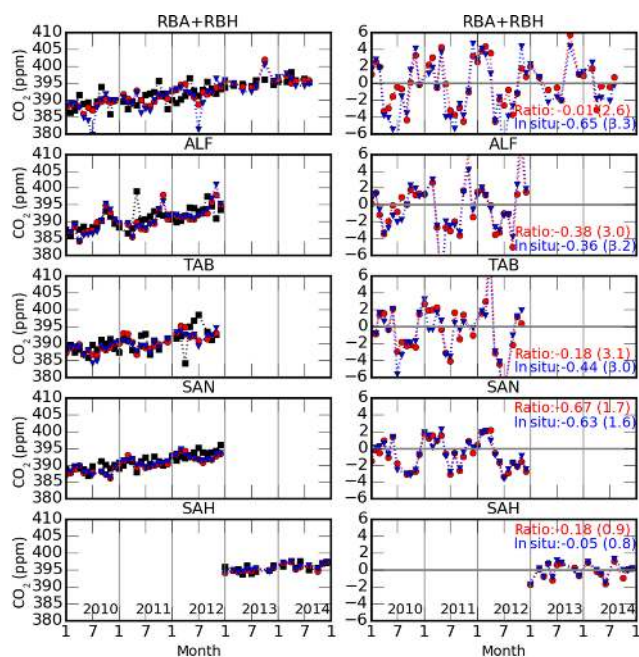
Figure 7. Monthly mean partial CO 2 columns at four sites over the Amazon (RBA, ALF, TAB, and SAN; Fig. 1) collected by the AMAZONICA project and two sites (RBH and SAH) after 2012 collected by the ACO project: comparison (left) and differences (right) with the GEOS-Chem model that has been sampled at the time and location of each observation and driven by fluxes inferred from the in situ (blue) and ratio (red) inversions. The mean and standard deviations (ppm) are shown in the inset of the right-hand-side panels. In the plot, we have combined the data over the AMAZONICA site RBA (for 2010 to 2012) and the ACO site of RBH (for 2012 to 2014) for a complete time series from 2010 to 2014 over the same location.
