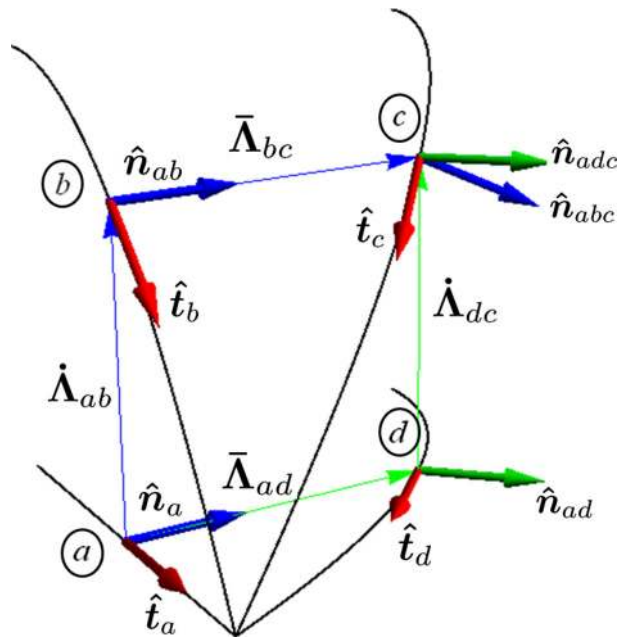
Fig. 1 Graphical interpretation of the nonvanishing connection symbol, corresponding to a rotation around the current unit tangent vector \hat{\boldsymbol{t}} (a torsional rotation)
