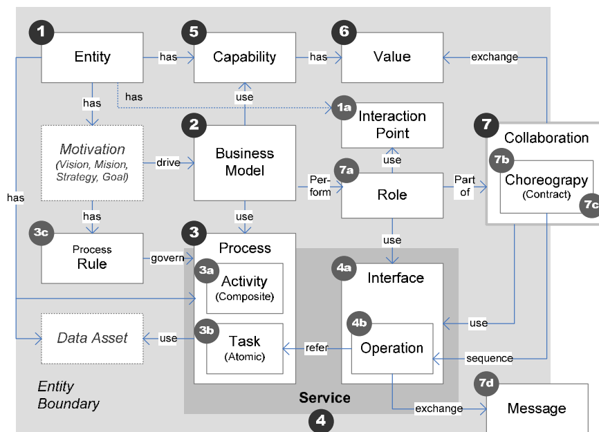
Fig. 9 General Service Engineering Ontology
