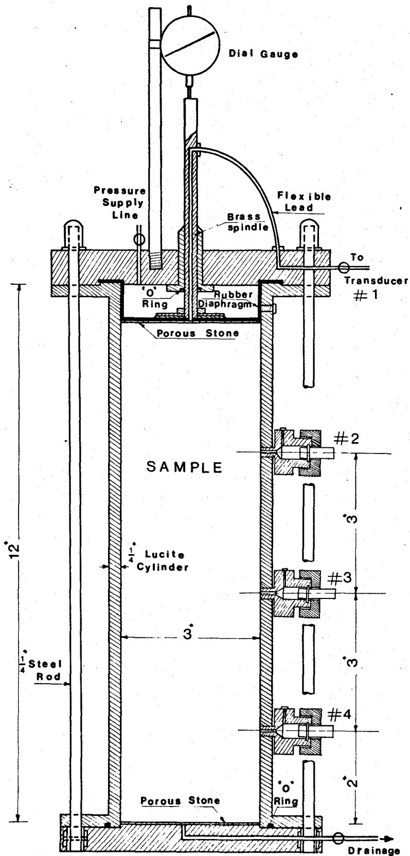
FIG.(11). THE CONSOLIDOMETER
