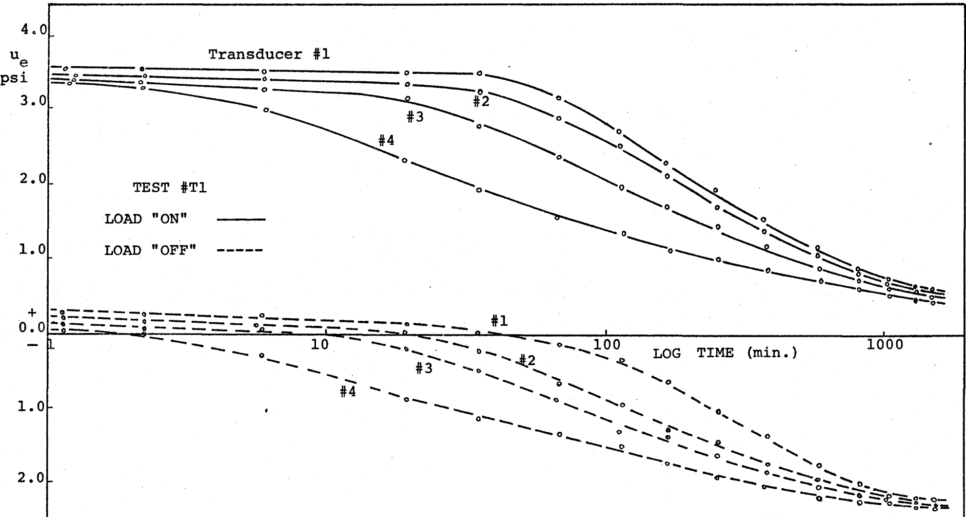
FIG. (14). EXCESS PORE WATER PRESSURE VERSUS TIME.
