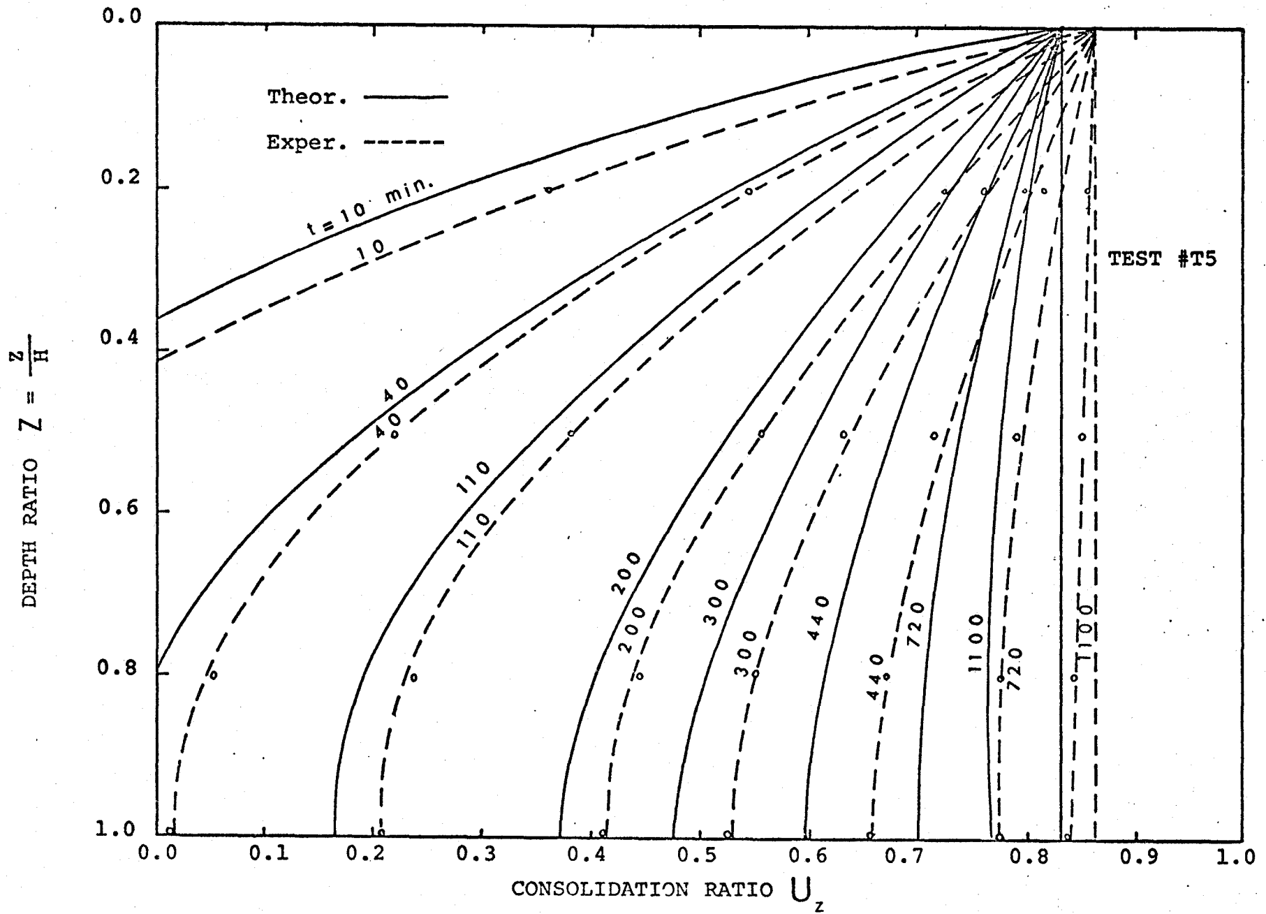
FIG. (19). CONSOLIDATION RATIO AS A FUNCTION OF DEPTH AND ELAPSED TIME.
