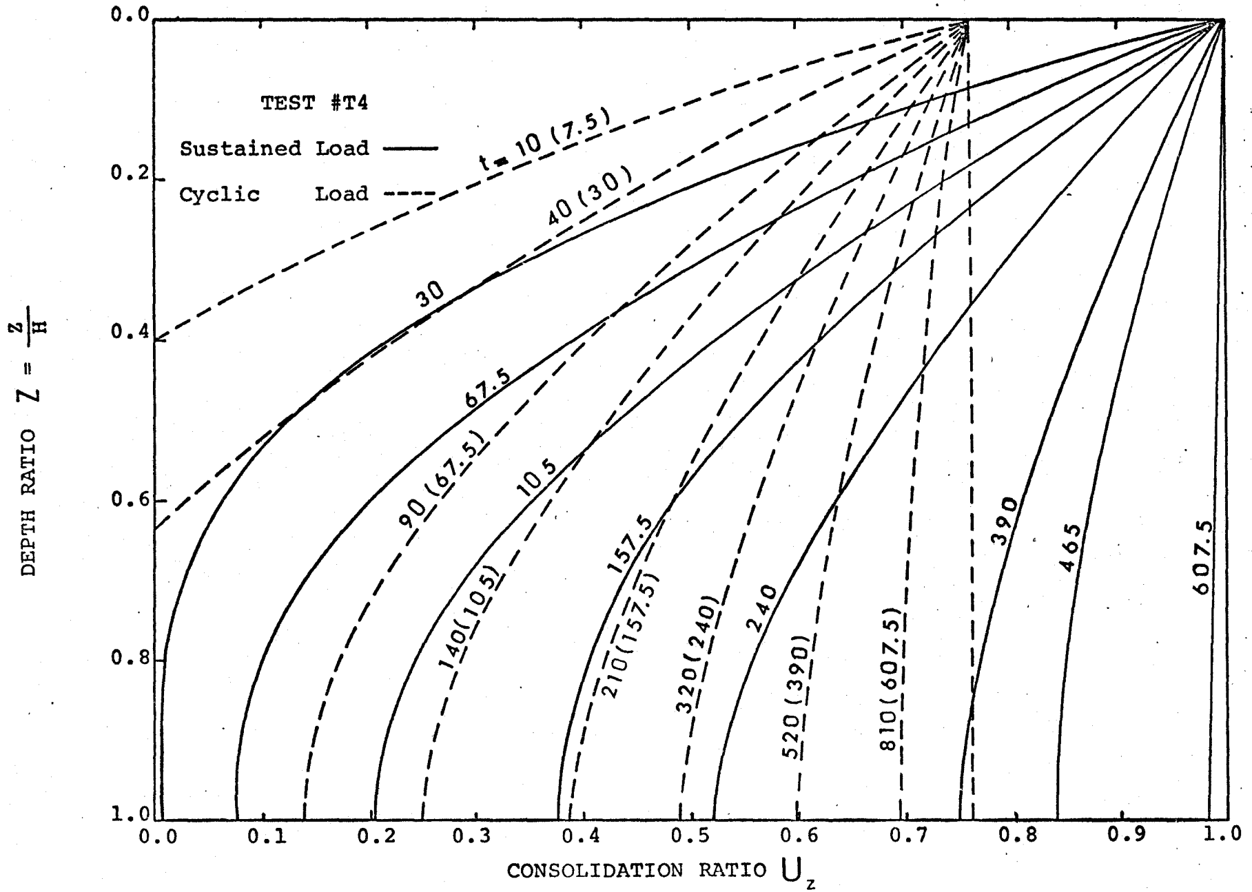
FIG. (21). COMPARISON BETWEEN CYCLIC AND SUSTAINED LOADING.
