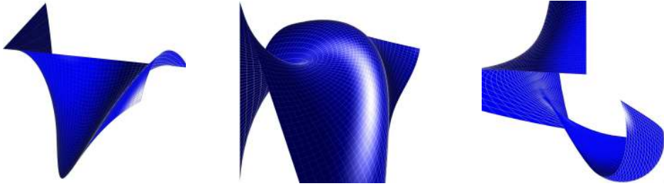
\mu=1, K=-1, \text{ target } \mathbb{E}^3 \mu=4, K=-\frac{16}{9}, \text{ target } \mathbb{S}^3 \mu=-4, K=\frac{16}{25}, \text{ target } \mathbb{S}^3
