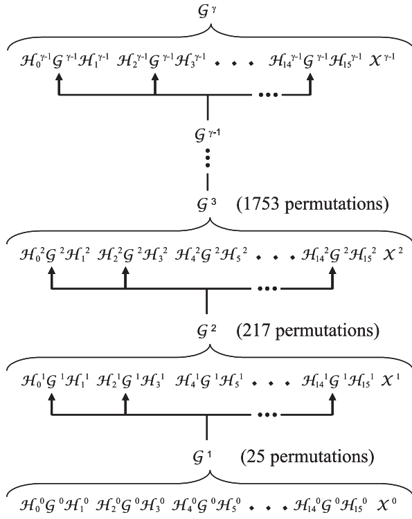
Figure 2. Structure of the order of the permutations in the MIN.
