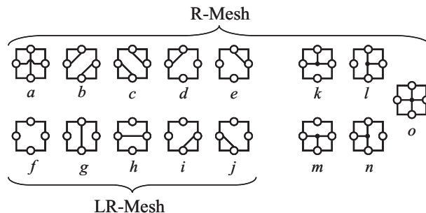
Figure 1. The possible internal connections of the R-Mesh and LR-Mesh.
