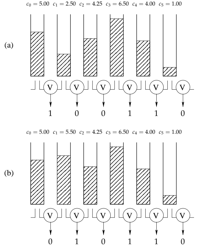
Figure 2. An example of a local “push-to-the-top” operation in a (1, 2, 6) -LRM scheme. The snapshot (a) presents the system before the change, while (b) presents the system after the change, which locally pushed c_1 above c_0 and c_2 , thus changing the first two bits of the demodulated sequence.
