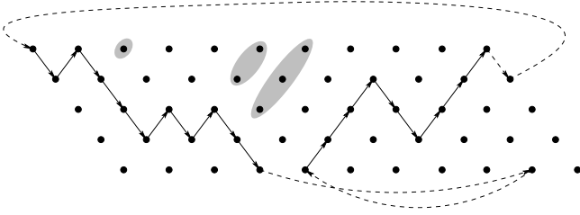
Figure 4. An example of a cyclic (1,2,11;2) -LRMGC. Solid arrows represent edges which are part of the up and down paths, and the shaded vertices are those which are guaranteed to remain uncovered in the proof of Theorem 11.
