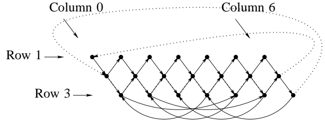
Figure 3. An example of an optimal non-cyclic (1, 2, 7; 2) -LRMGC which results from Construction 1. Solid arrows represent edges which are part of the code path, while dotted arrows represent those that are not.
