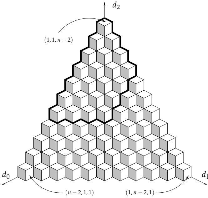
Figure 5. The hyperplane of configurations for n = 13 . The set of canonical configurations is shown surrounded by a thick frame.
