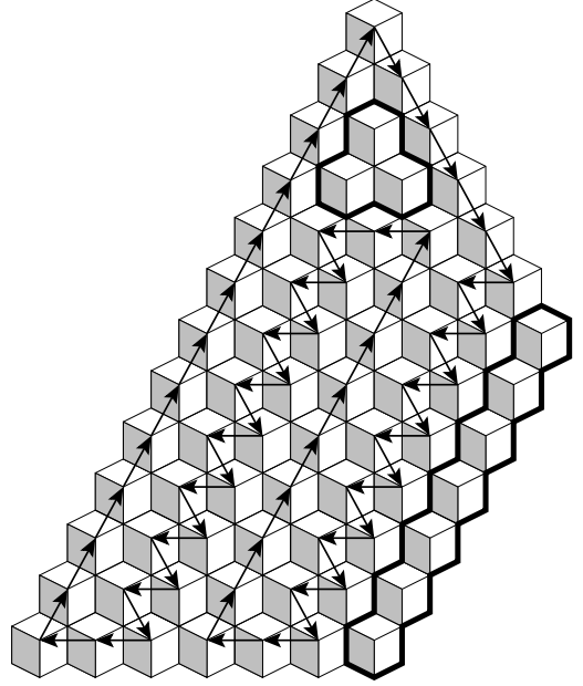
Figure 6. The path from Construction 2 over the canonical configurations for n = 22 . The unvisited configurations are shown surrounded by a thick frame.
