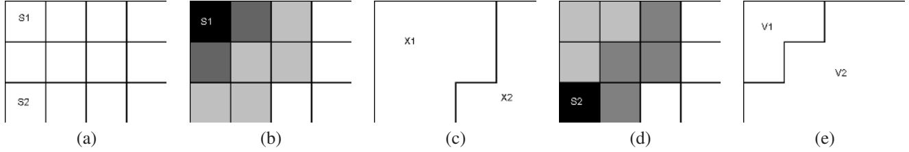
Figure 3. Example of classical metric tessellations on the ultrametric space of Figure 2. (a): two sites s_1 and s_2 . (b): distance to s_1 . (c): Tessellation obtained by thresholding the distance to s_1 at level 3. (d): distance to s_2 . (e): Voronoi tessellation with respect to the two sites. Note that (e) cannot be obtained by thresholding the UCM at a constant level.
