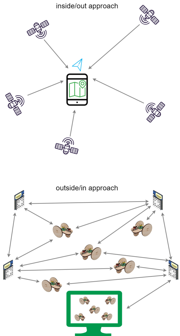
FIGURE 4. Localization architecture approaches: inside/out (top) and outside/in (bottom).
