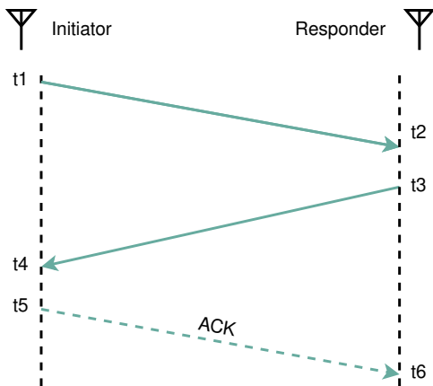
FIGURE 2. Time of Flight technique.
