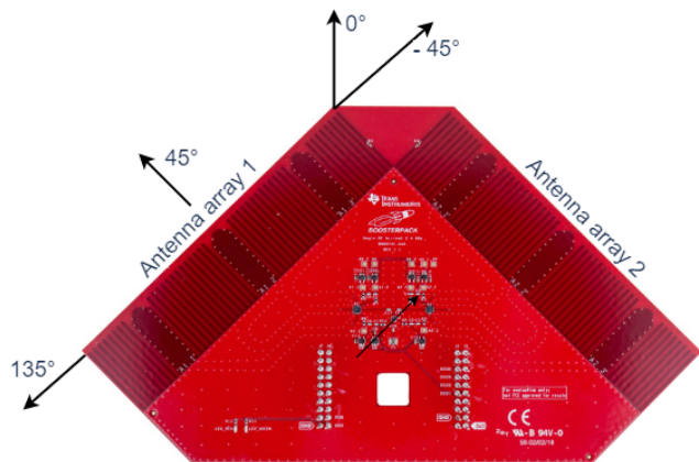
FIGURE 6. BOOSTXL-AOA antenna array from Texas Instruments.
