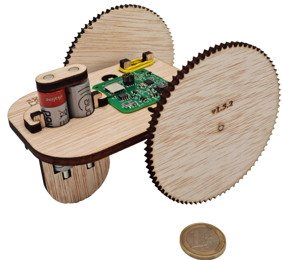
FIGURE 1. DotBot - low-cost, small form-factor micro robot for educational and research purposes in networking and swarm robotics.
