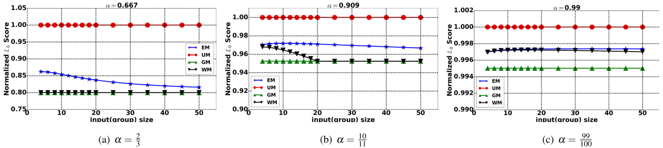
Fig. 9. Final groups of mechanisms with distinct behaviors.
