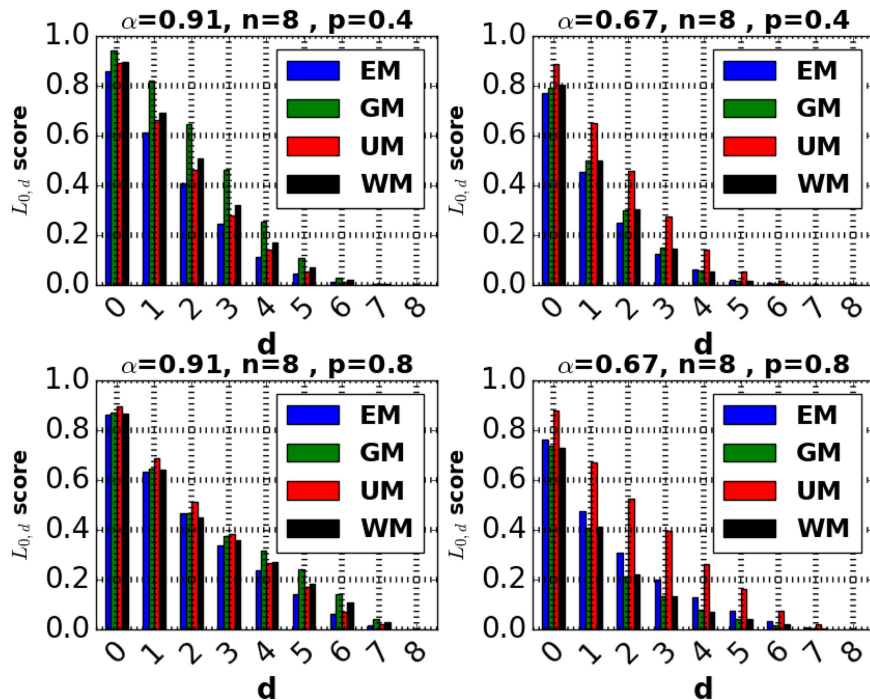
Fig. 12. Histograms of L_{0,d} scores for Binomial data.
