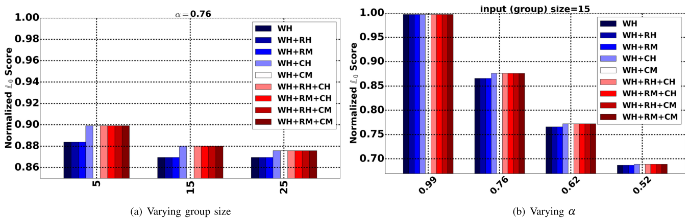
Fig. 8. Combinations of properties with weak honesty.
