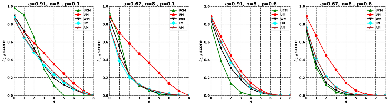
Fig. 18. Line plots for \mathbb{L}_{2,d} scores for Binomial data ( p = 0.1 and p = 0.6 ).
