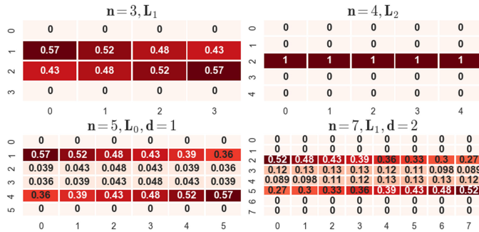
Fig. 1. Heatmaps of unconstrained mechanisms for \alpha = 0.62 .
