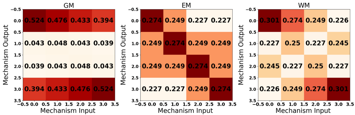
Fig. 7. Heatmaps for GM, EM, and WM with n = 4 .
