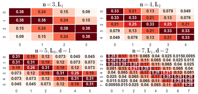
Fig. 2. Heatmaps of constrained mechanisms for \alpha = 0.62 .
