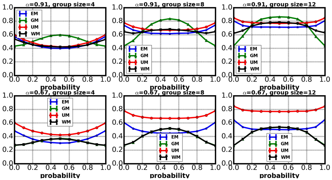
Fig. 11. L_{0,1} score for Binomial data, for n = \{4, 8, 12\} and \alpha = \{0.91, 0.67\} .
