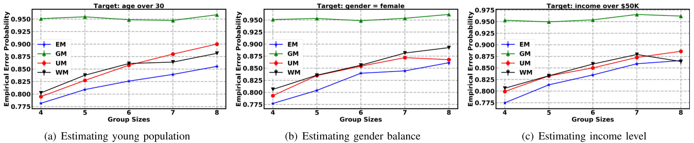
Fig. 10. Empirical error probability on adult dataset for \alpha = 0.9 .
