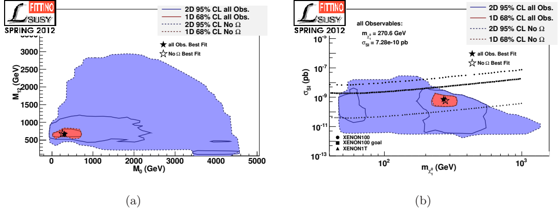
Figure 19. Solid lines show the standard LHC fit, dashed lines the impact of the relic density constraint on (a) the (M_0, M_{1/2}) plane and (b) \sigma_{\text{SI}} vs. m_{\tilde{\chi}_1^0} . In (b) also the current (Xenon100) as well as near (XENON100Goal) and far (XENON1T) future reaches of direct detection experiments are shown (from top to bottom).
