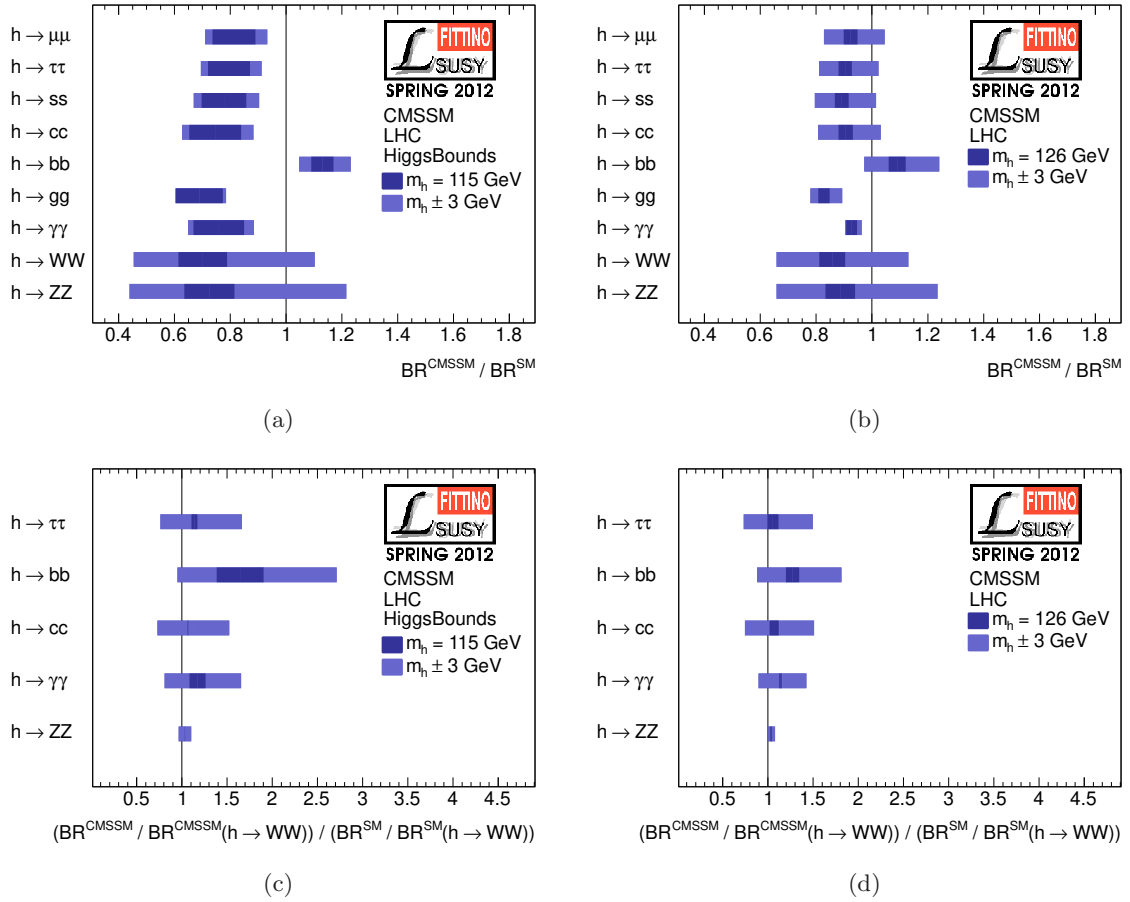
Figure 14. Predicted 2\sigma range of Higgs branching fractions for the LHC fit of the CMSSM in (a) and the CMSSM fit with m_h = (126 \pm 2 \pm 3) GeV in (b). The results do include the theoretical uncertainty of the Higgs boson mass of \pm 3 GeV. Ratios of the potentially experimentally accessible branching fractions at LHC are given in in (c) and (d) for the same fits as above.
