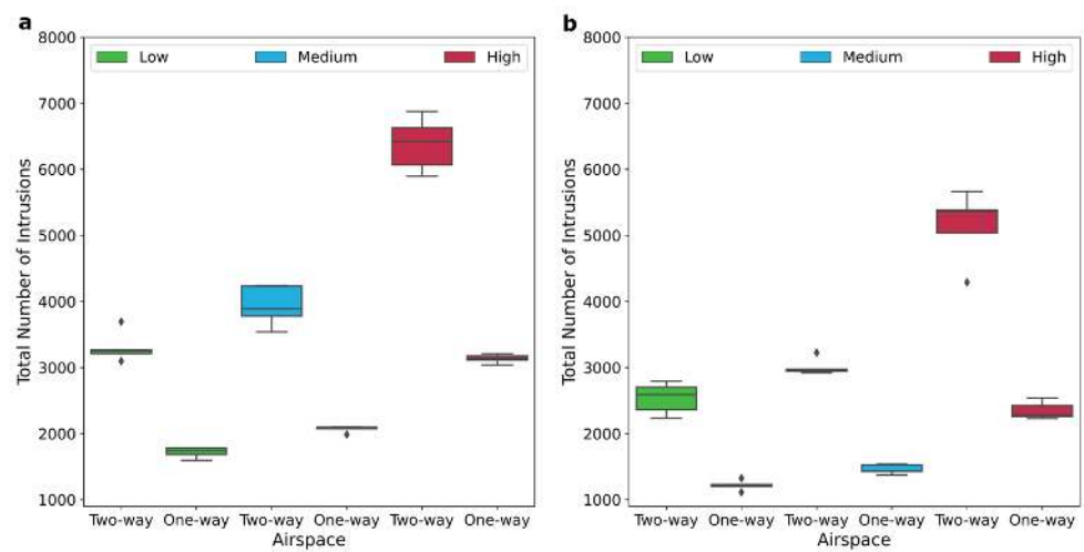
Figure 8. The total number of pairwise intrusions for the two-way and one-way urban airspace concept for low, medium, and high traffic demands. (a) Without conflict resolution. (b) With conflict resolution.
