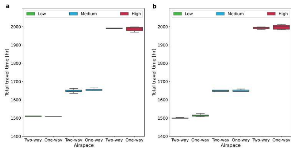
Figure 12. The total travel time for the two-way and one-way urban airspace concept for low, medium and high traffic demands. (a) Without conflict resolution. (b) With conflict resolution.
