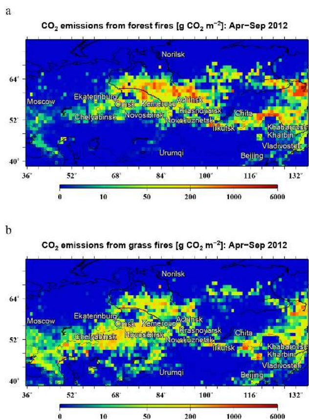
Figure 4. CO 2 biomass burning emissions ( \text{g CO}_2 \text{m}^{-2} ) from (a) forests and (b) from other types of vegetative land cover (mainly grasslands): mean values estimated in this study for the period from April to September 2012.
