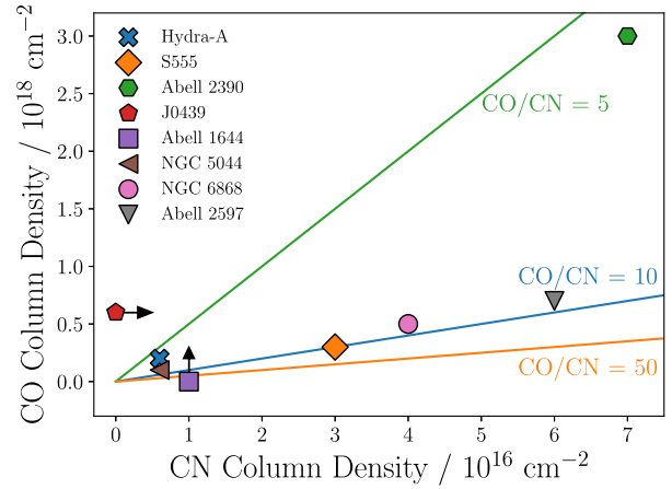
Figure 6. The total line-of-sight CO and CN column densities of the absorption regions shown in Figs 2 and 3, values of which are given in Table 6. These are mostly derived from the integrated optical depths shown in Table 5 and Fig. 5. However, for NGC 5044 and Abell 2597, we use archival CO(2–1) observations which show the absorption more clearly. The column densities are calculated using equation (1) and assuming a gas temperature of 40 K. For most sources, the CO/CN ratio is 10.
