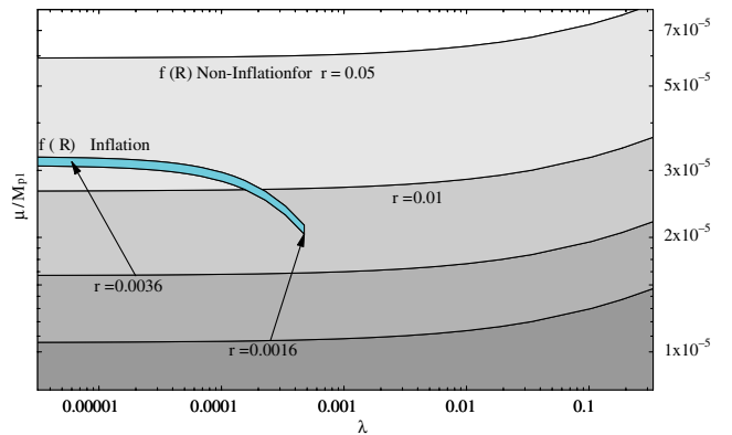
FIG. 4 (color online). Constraints on the cubic f(R) model. The thin gray (blue) sliver corresponds to observationally allowed f(R) inflationary scenarios. Shaded are regions we may rule out given a measurement of the tensor to scalar ratio r and the assumption that they were generated by a period of slow-roll inflation in the early universe. The r = 0.05 and r = 0.01 are the most realistic curve, in the sense that future experiments are sensitive to such values as low as r = 0.01 [56].
