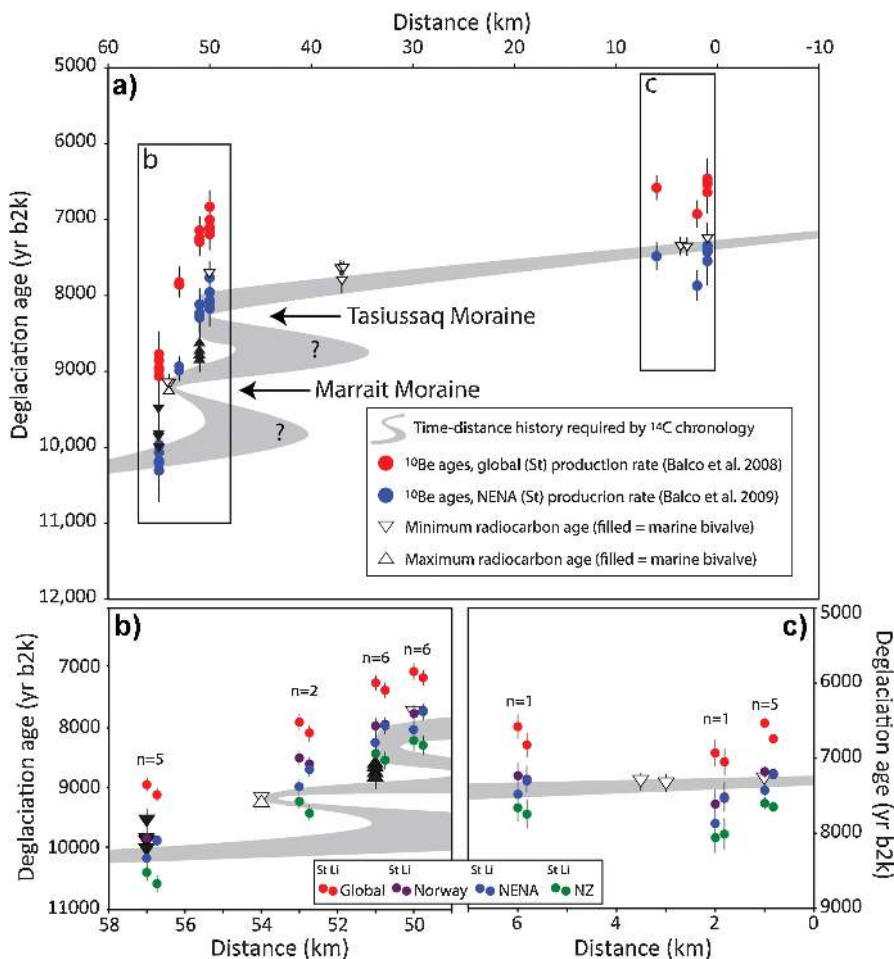
Figure 3. (a) Time–distance history of Jakobshavn Isbrae between the coast of Disko Bugt and the present ice margin. Distance is simplified; the broader area north and south of Jakobshavn Isfjord is condensed into a single distance profile through the Isfjord. Grey shaded line is the time–distance history required by the radiocarbon ages. (b,c) Enlarged portions of the diagram in (a), showing only the average age per ice margin position. Two adjacent symbols represent the Lal/Stone (St) and Lifton (Li) scaling schemes; the two adjacent symbols are measurements from the same ice margin position. We add the age solutions using the ^{10}\text{Be} production rates from New Zealand (Putnam et al. , 2010) and southern Norway (Goehring et al. , 2012); see supporting Table S3. Sample error bars include one-sigma analytical uncertainty.
