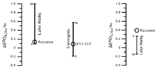
Figure 10. Comparison of isotopic changes in speleothems ( \Delta\delta^{18}O_{C\_spel} ) for the 8.2 ka event (left) and 3.2 ka event (right) in stalagmites from Ascunsă and V11 caves with pollen temperature-constrained range of \Delta\delta^{18}O_{C\_pct} (summer and winter) calculated by using data from Steregoiu peat bog (Feurdean et al., 2008 and Lake Maliq (Bordon et al., 2009).
