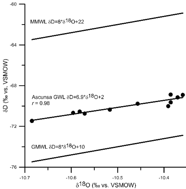
Figure 6. Comparison between global meteoric water lines (GMWL; Craig, 1961) and Mediterranean meteoric water lines (MMWL; Gat and Carmi, 1970), as well as Ascunsa Cave groundwater line.
