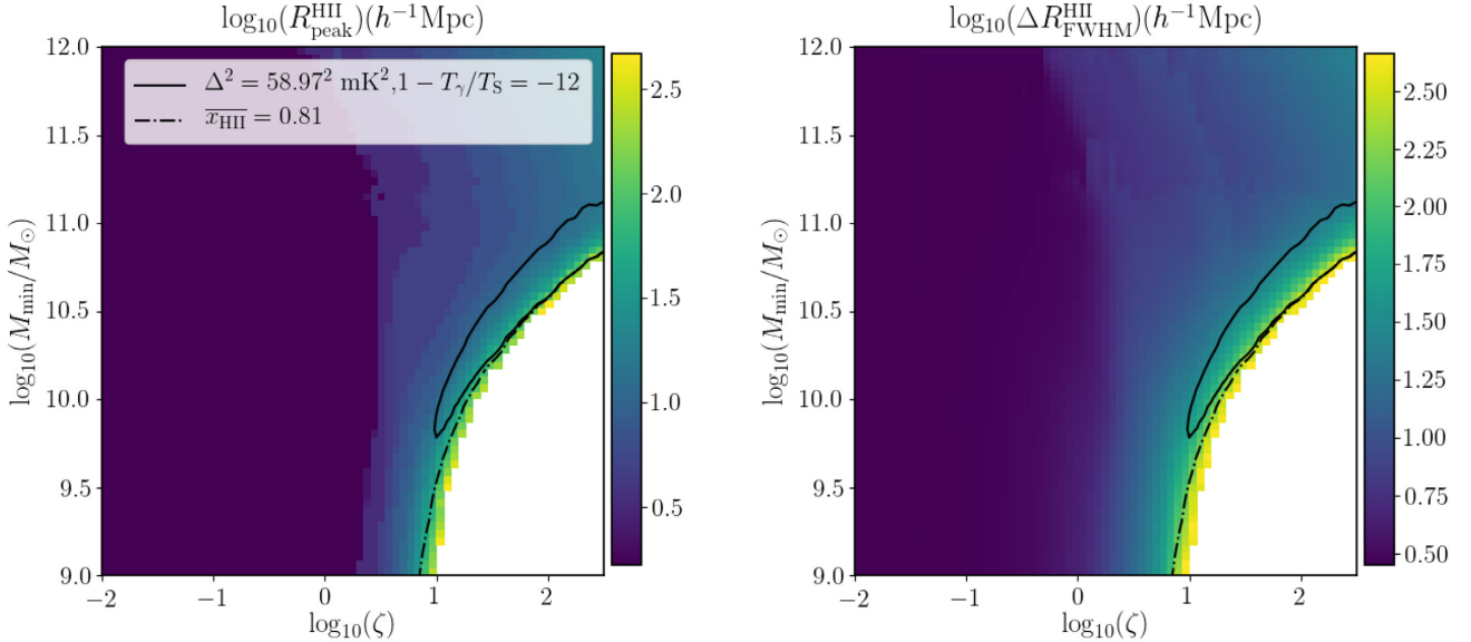
Figure 5. The distribution of R_{\text{peak}}^{\text{HII}} (left-hand panel) and \Delta R_{\text{FWHM}}^{\text{HII}} (right-hand panel) over the parameter space of \zeta and M_{\min} for z \approx 9.1 . R_{\text{peak}}^{\text{HII}} and \Delta R_{\text{FWHM}}^{\text{HII}} represent the radius at which the probability distribution of the sizes of the ionized regions has maximum amplitude and the FWHM of that distribution, respectively. We use the MFP method to estimate the bubble size distribution. The region in white in the bottom right of the panels corresponds to fully ionized IGM at redshift \approx 9.1 . The solid curves show the contours of \Delta^2 = (58.97)^2 \text{ mK}^2 for 1 - T_{\gamma}/T_S = -12 . For a deterministic observation, the region enclosed by the solid contour will be excluded. The dash-dotted line shows the contour for \bar{x}_{\text{HII}} = 0.81 .
