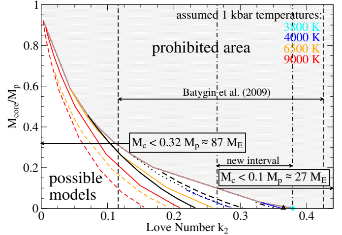
Fig. 2. Love numbers k_2 and core masses of two-layer models of HAT-P-13b for different 1 kbar temperatures (color coded). For pressures < 1 kbar the temperature profile is either adiabatic (colored solid) or isothermal (colored dashed). The metallicity increases along a line, reaching its maximum value for M_{\text{core}}/M_p = 0 . The zero metallicity line for fully adiabatic models (brown solid) separates the region of all possible planetary models (white) from the prohibited area (light gray). Vertical black dashed lines indicate the allowed interval for k_2 -values derived by BBL. Based on that interval we find a maximum possible core mass of 0.32 M_p \approx 87 M_\oplus . Our new k_2 interval is shown with vertical black dot-dashed lines. It lowers the uncertainty of the planet's core mass down to 0.1 M_p \approx 27 M_\oplus . The other black lines show our models that are based on our model atmosphere with a fully adiabatic envelope (solid black) and P_{\text{ad}} of 5 bar (dotted black), 10 bar (dashed black), 50 bar (dot-dashed black), and 72 bar (black triangle).
