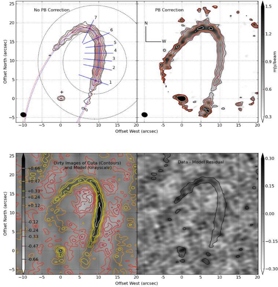
Fig. 1.— Top-left : 350 GHz ALMA image of Fomalhaut’s ring. The RMS noise is \sim 60 \mu\text{Jy beam}^{-1} , and the contours represent 0.24, 0.33, 0.47, 0.66, 0.92, and 1.4 \text{mJy beam}^{-1} . The circles are centered on the pointing center, and their diameters show the beam’s half and 7% power. Ellipses with \text{PA} = 336^\circ , and i = 66^\circ (red) and 67^\circ (blue) are shown, with the ellipse centers given by the plus sign. The slices labeled 1-7 are used to show surface brightness profiles in Figure 2. The coordinate axis is centered on the star, which has a peak brightness of 0.49 \text{ mJy beam}^{-1} (uncorrected). Top-right : The primary beam corrected image. The ring becomes bright near the ansa , and remains bright through the inferred apocenter. The contours are the same as in the top-left, but begin at 0.47 \text{ mJy beam}^{-1} . Bottom-left : The best-fit skymodel is compared with the dirty ALMA image. The grayscale and contours show \text{mJy beam}^{-1} , with the contour levels labeled on the colorbar. Bottom-right : The residual of the data minus the model. The model subtracts the emission well, but there remains excess emission in the NE and around the star.
