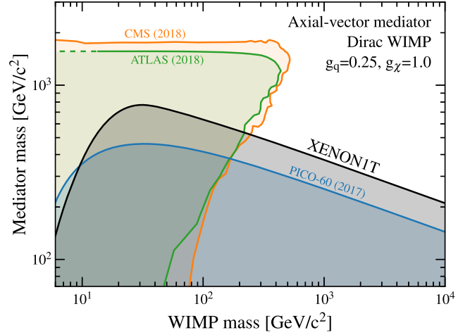
FIG. 4. XENON1T 95% C.L. upper limit in the m_{\text{med}} - m_\chi plane for a simplified isoscalar model with an axial-vector mediator and a Dirac WIMP, where the mediator-quark ( g_q ) and mediator-WIMP ( g_\chi ) couplings are fixed to 0.25 and 1.0, respectively. Shown for comparison are 95% C.L. limits from PICO-60 [38], ATLAS [40], and CMS [41]. The shaded regions are excluded by the correspondingly colored limits.
