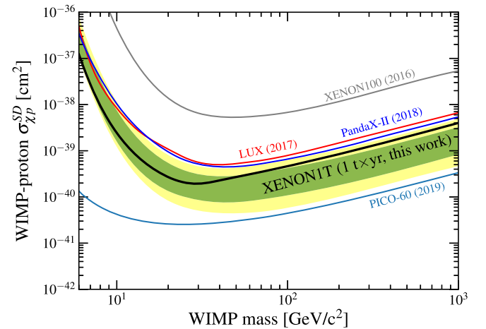
FIG. 3. XENON1T 90% C.L. upper limit on the spin-dependent WIMP-proton cross section from a 1 ton year exposure. The range of expected sensitivity is indicated by the green ( 1\sigma ) and yellow ( 2\sigma ) bands. Selected experimental results are shown for XENON100 [24], LUX [25], PandaX-II [26], and PICO-60 [34]. We use the chiral EFT limit from PandaX-II, since it is based on the same SD interaction model as all other shown results.
