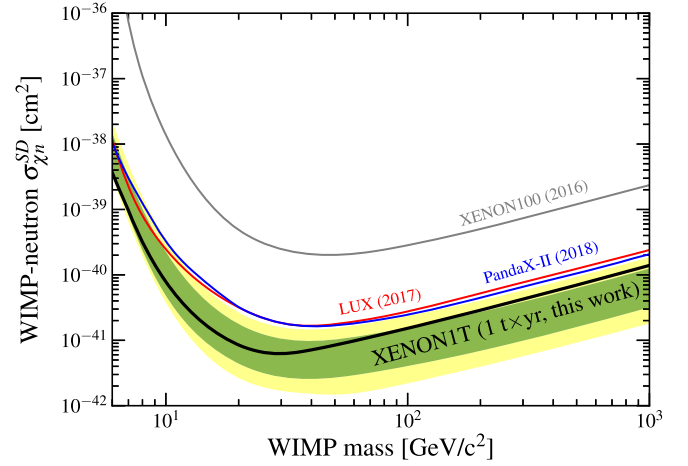
FIG. 2. XENON1T 90% C.L. upper limit on the spin-dependent WIMP-neutron cross section from a 1 ton year exposure. The range of expected sensitivity is indicated by the green ( 1\sigma ) and yellow ( 2\sigma ) bands. Also shown are the experimental results from XENON100 [24], LUX [25], and PandaX-II [26]. We use the “chiral EFT” limit from PandaX-II, since it is based on the same SD interaction model as all other shown results.
