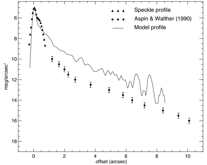
Fig. 11. K band profile along the cavity axis for IRS3 S. The speckle data (filled triangles) are obtained from Fig. 10b. The solid circles represent the data from the contour map shown by Aspin & Walther (1990). The solid line corresponds with an extension of the fiducial model up to a radius of 9.4 \times 10^4 AU. The speckle data and the model are flux calibrated following the procedure explained in the text. The offsets are in arcseconds from the position of the star. The errors for the speckle data are smaller than the size of the plotting symbol.
