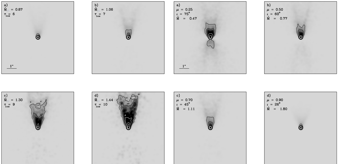
Fig. 1. K band images for models in which the infall rate has been varied with respect to the fiducial model (K01 in Table 1, see Fig. 2c). a) Model K02 with a 0.87 \times 10^{-4} M_{\odot} \text{ yr}^{-1} . b) Model K03 ( 1.06 \times 10^{-4} M_{\odot} \text{ yr}^{-1} ). c) Model K04 ( 1.30 \times 10^{-4} M_{\odot} \text{ yr}^{-1} ). d) Model K05 ( 1.44 \times 10^{-4} M_{\odot} \text{ yr}^{-1} ). The rest of the parameters remain unchanged with respect to model K01. In the four panels, the line of sight forms an angle of 45^{\circ} with respect to the cavity axis. The 1'' bar represents a length of 1000 AU, and the resolution used is 0''.2 . The greyscale varies from -5\% (the lightest) to 20\% of the maximum brightness (the darkest). The contours are at 5, 10, 15, 30 and 50% of the maximum brightness. These contour levels have been chosen for comparison with typical near-IR speckle imaging in 4 m-class telescopes (see Paper I). \tau_{\text{los}} represents the optical depth along the line of sight. These and the other model images shown in this section are normalised to the brightness peak, unless otherwise stated.
