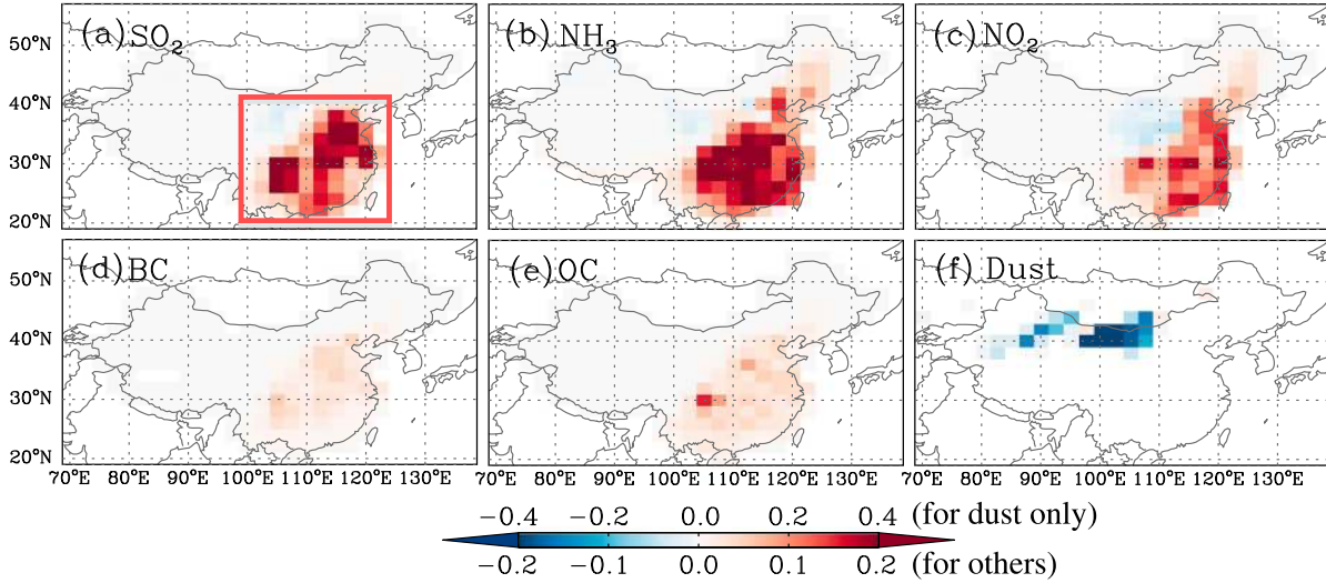
Figure 2. Relative changes in posterior aerosol emissions from a priori in the pseudo-observation experiment. Six panels are, respectively, for anthropogenic emissions of \text{SO}_2 , \text{NH}_3 , \text{NO}_x , BC, and OC, and mineral dust from both natural and anthropogenic sources. The red box in Figure 2a indicates the region where AOD observations are selected.
