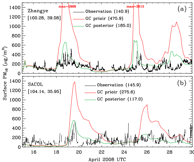
Figure 11. Time serial plot of the GEOS-Chem-simulated surface PM10 concentrations by prior (red) and posterior (green) aerosol emissions compared with the in situ measured PM10 (black) over (a) Zhangye and (b) SACOL stations for 15–30 April 2008; also shown are the average values over same the period. Discontinuity in time series is due to missing or quality filtered observations.
