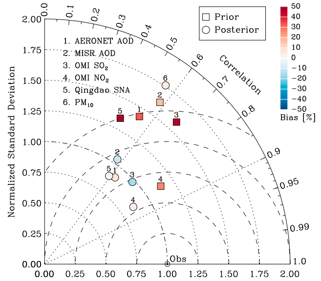
Figure 12. Taylor diagram for the model evaluations before (squares) and after (circles) optimization when comparing against (1) AERONET AOD at 0.55 \mu\text{m} , (2) MISR 0.55 \mu\text{m} AOD, (3) OMI column \text{SO}_2 , (4) OMI column \text{NO}_2 , (5) surface SNA concentrations at Qingdao site, and (6) surface \text{PM}_{10} concentrations measured at Zhangye and SACOL sites. The color coded on each point indicates the relative bias. It should be noted that the ratio of standard deviations and correlation coefficient between prior GEOS-Chem-simulated and measured surface \text{PM}_{10} over Zhangye and SACOL is 6.5 and 0.45, which makes the point number 6 for the prior simulation far beyond the range of this Taylor diagram.
