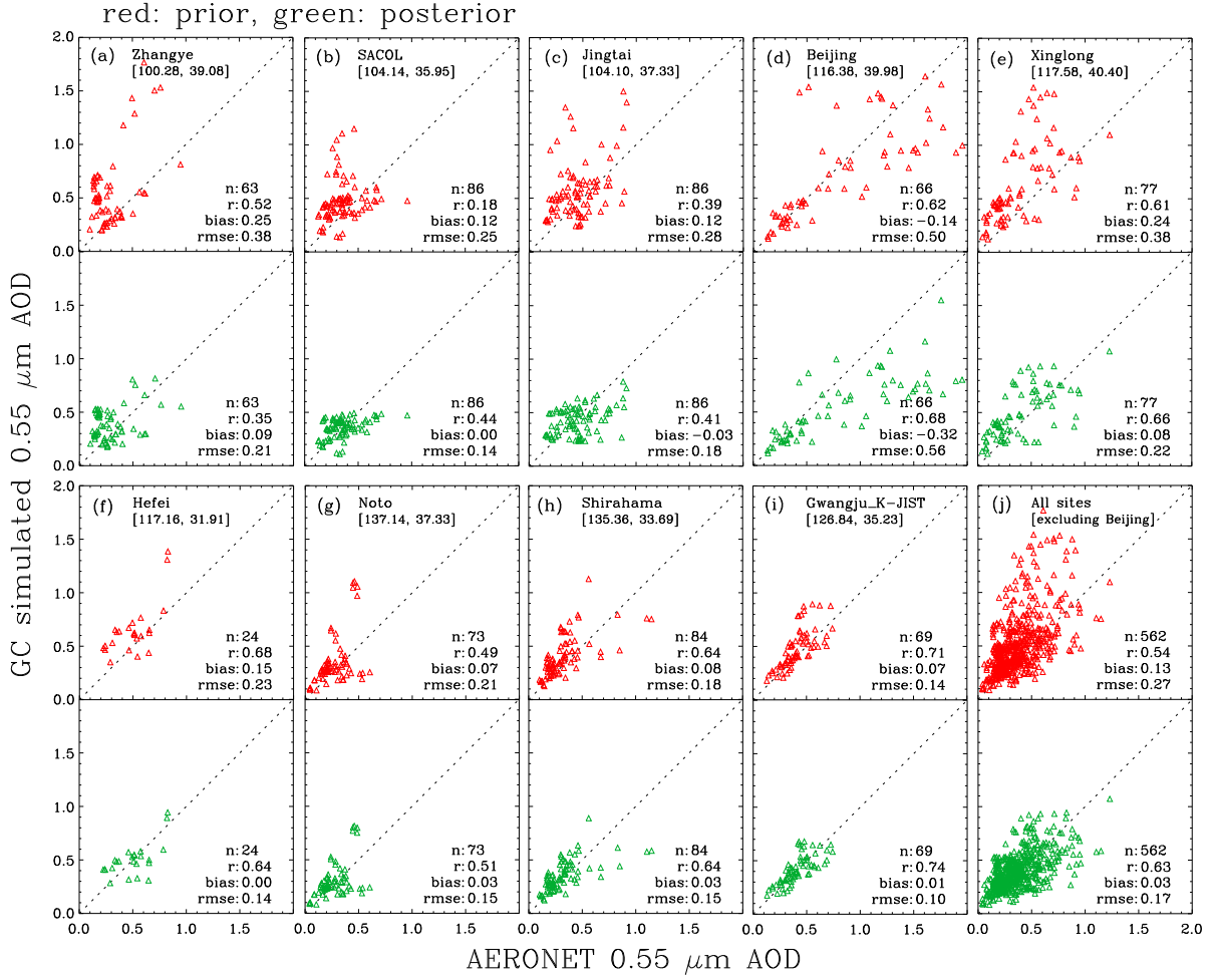
Figure 6. (a – i) Scatterplots of GEOS-Chem AOD versus AERONET AOD at 0.55 \mu\text{m} prior (red scatters) and posterior (green scatters) to the aerosol emission optimization over nine stations. AERONET AODs are 3 h averages following the GEOS-Chem output frequency. (j) The overall comparison for eight AERONET sites excluding Beijing. Also shown are the number of valid sampled pairs ( n ), correlation coefficients ( R ), bias, and root-mean-square-error (RMSE).
