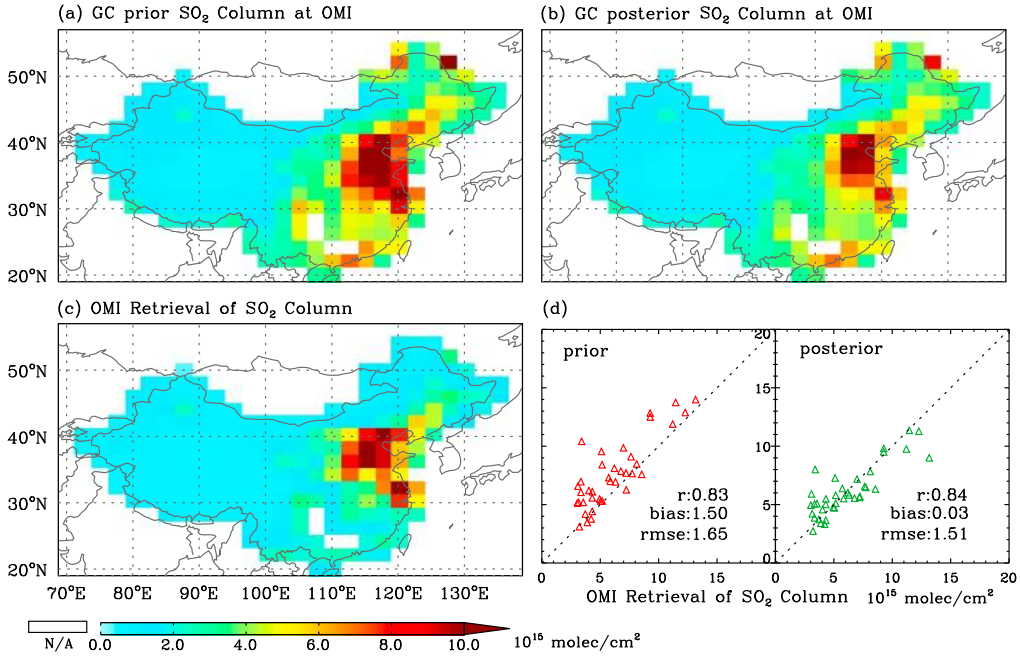
Figure 8. Same as Figure 7 but for comparison of the GEOS-Chem \text{SO}_2 simulation with OMI column \text{SO}_2 retrievals for the period of April 2008. The OMI planetary boundary layer (PBL) column \text{SO}_2 from the Level 3 daily products with 0.25^\circ \times 0.25^\circ resolutions are aggregated into GEOS-Chem grid cells.
