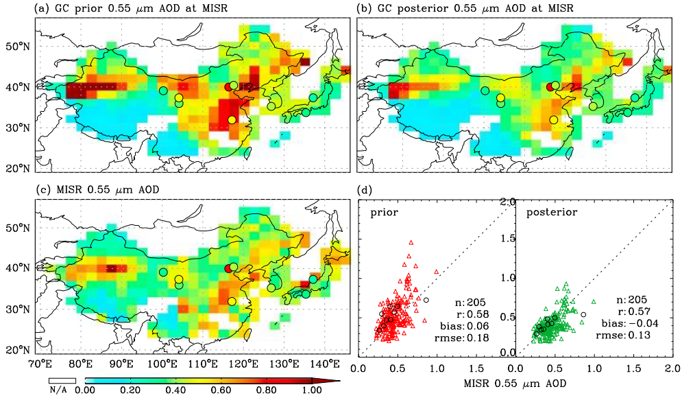
Figure 7. Comparison of the prior and posterior GEOS-Chem simulation of 0.55 \mu\text{m} AOD with the Level 3 MISR 0.55 \mu\text{m} AOD for the period April 2008. (a) The prior GEOS-Chem 0.55 \mu\text{m} AOD that are sampled coincidentally with MISR AODs for the period of April 2008. Also overlaid circles are the monthly AOD averages at 0.55 \mu\text{m} observed from the nine AERONET sites shown in Figure 5. Figure 7(b) Same as Figure 7a but for the monthly average of posterior GEOS-Chem AOD. (c) Monthly average of the Level 3 daily MISR 0.55 \mu\text{m} AOD. (d) Scatterplot of the GEOS-Chem AOD versus the MISR AOD before (red scatters) and after optimization (green scatters), in which each point indicates an AOD pair over a model grid cell with value over 0.2. Also shown are the statistics including number of sampled pairs (n), correlation coefficient (R), bias and root-mean-square-error (RMSE). Comparisons of the monthly GEOS-Chem AOD versus AERONET AOD are also included as the black circles; each circle indicates an AOD pair over an individual site.
