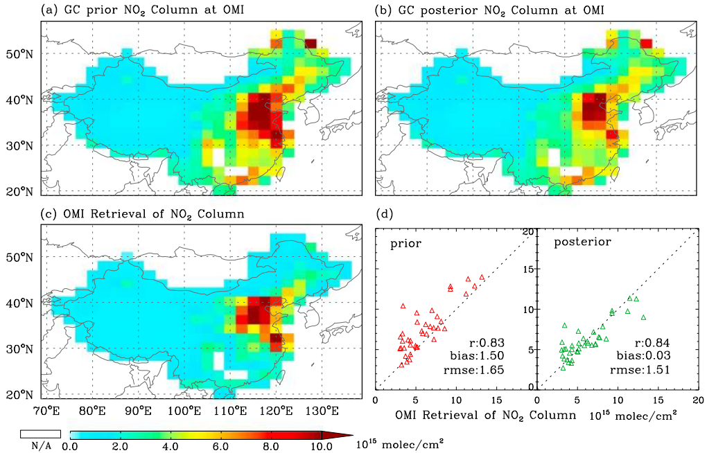
Figure 9. Same as Figure 7 but for comparison of the GEOS-Chem \text{NO}_2 simulation with OMI column \text{NO}_2 retrievals for the period of April 2008. The OMI tropospheric column \text{NO}_2 from Level 2 daily products with 0.25^\circ \times 0.25^\circ resolutions are aggregated into GEOS-Chem grid cells.
