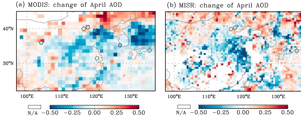
Figure 13. Change of April monthly 0.55 \mu\text{m} AOD from 2006 to 2008 from (a) MODIS and (b) MISR Level 3 daily products.
