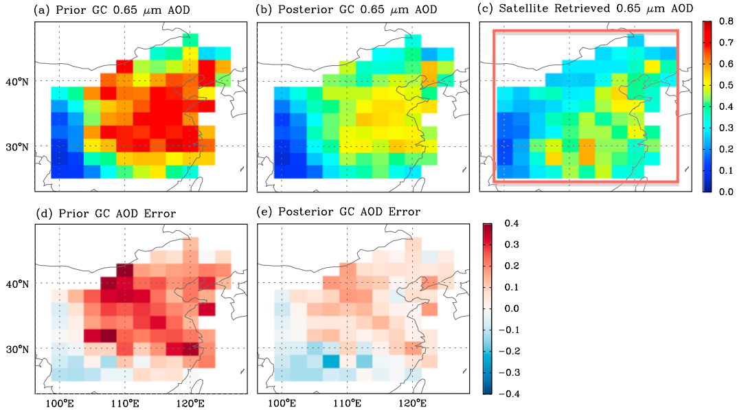
Figure 3. Comparison of the (a) prior and (b) posterior GEOS-Chem (GC) simulation of 0.65 \mu\text{m} AOD with the AOD at the same wavelength retrieved from MODIS reflectance using GEOS-Chem aerosol optical properties (c) averaged for the period of April 2008. Satellite retrievals with 10 \text{ km} \times 10 \text{ km} at nadir are aggregated to GEOS-Chem grid cells; and the model AOD are sampled coincidentally with those retrievals. Figure 3d and 3e, respectively, show the difference of prior and posterior simulated from the satellite retrieved AODs. The red box in Figure 3c indicates the region where AOD observations are selected.
