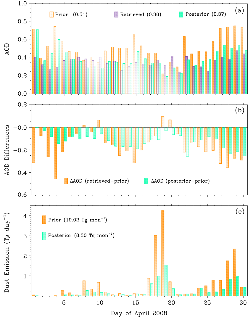
Figure 4. (a) Time series of the spatially averaged daily MODIS AOD retrievals (purple) for April 2008 over the Eastern China, compared by the prior (orange) and posterior (green) spatially averaged daily GEOS-Chem AOD that are sampled in the MODIS AOD tempo-spatial space. (b) Time series of the expected daily AOD adjustments (orange) that are the differences between MODIS AOD and the prior GEOS-Chem AOD and their real adjustments (green) that are the differences of posterior from prior GEOS-Chem AOD. (c) Time series of the prior (orange) and posterior (green) daily dust emissions over China for April 2008.
