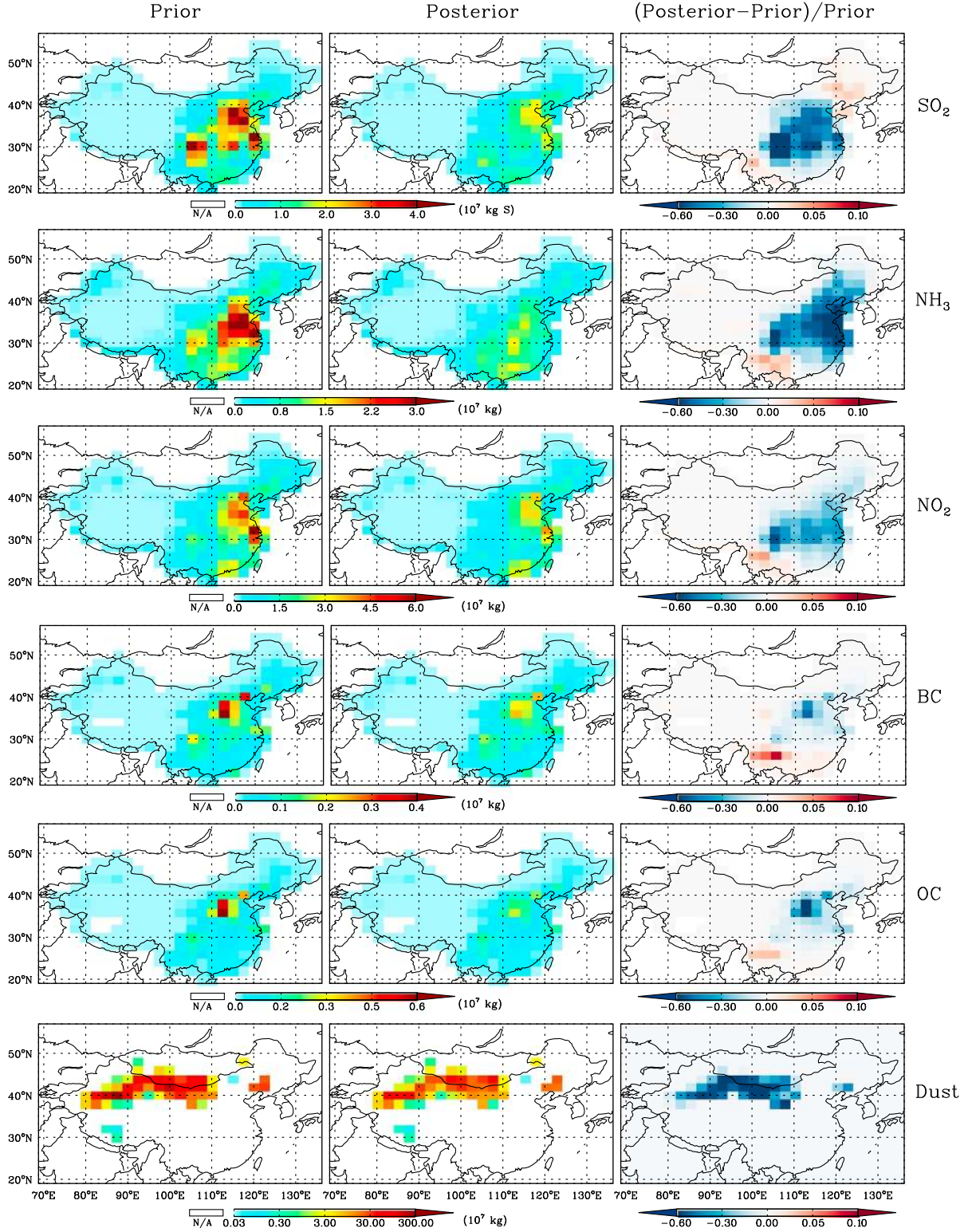
Figure 5. The prior (or bottom-up based, left column), optimized (or top-down constrained, middle column) aerosol emissions over China for the period of April 2008, and their relative differences (right column). Six rows from top to bottom are, respectively, for anthropogenic emissions of \text{SO}_2 , \text{NH}_3 , \text{NO}_x , BC, and OC, and mineral dust from both natural and anthropogenic sources.
