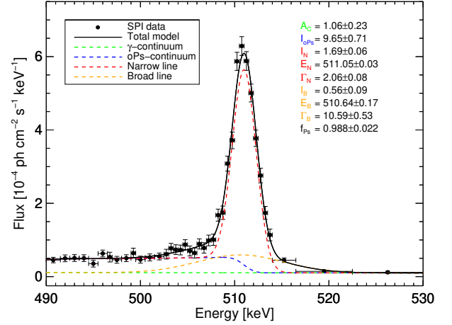
Fig. 1. Positron annihilation spectrum of the Galaxy using the best-fit morphology model of Siegert et al. (2016). Shown are the SPI data points in black ( \geq 3\sigma -bins), and four model components: narrow 511 keV line (red), broad 511 keV line (orange), ortho-positronium continuum (blue), galactic \gamma -ray continuum (green). The total model is shown as solid black line. The fitted parameters are shown in the legend. The units are 10^{-5} ph \text{cm}^{-2} \text{s}^{-1} \text{keV}^{-1} for the continuum amplitude A_C , 10^{-3} ph \text{cm}^{-2} \text{s}^{-1} for the line fluxes I_N and I_B , and the positronium continuum I_{\text{oPs}} , and keV for the lines centroids E_N and E_B , and widths \Gamma_N and \Gamma_B . The positronium fraction f_{\text{pS}} is measured to be between 0.97 and 1.00.
