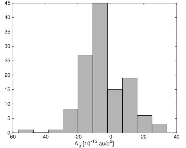
Fig. 1. Histogram of Yarkovsky estimates normalized by an absolute magnitude scale factor of 1329 \text{ km } 10^{-H/5} / \sqrt{0.154} . The average 1\sigma uncertainty in normalized A_2 is 5 \times 10^{-15} \text{ au/d}^2 .
