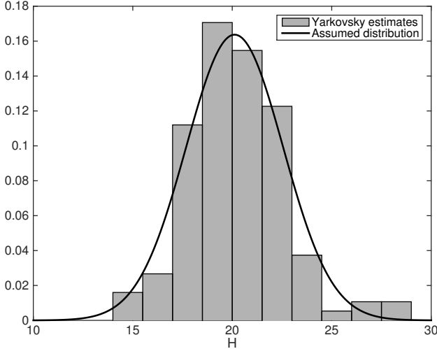
Fig. 2. Probability distribution of the absolute magnitude for the objects in Table A.1.
