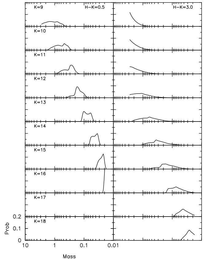
FIG. 13.—Illustrative mass probability functions derived using our methodology. The left panels show stars with H-K = 0.5 and the right panels show stars with H-K = 3.0 , both columns of panels decreasing in brightness top to bottom from K = 9 to K = 18 . The dereddening model uses the same distributions in age and in near-infrared excess as employed elsewhere in this paper. Note the tails upward at the lower and upper mass extrema in the panels for K = 16 , H-K = 0.5 and K = 9 , H-K = 3.0 , respectively. These are caused by our imposition of integrated probability equal to unity over the mass range 0.02-3.0 M_\odot .
