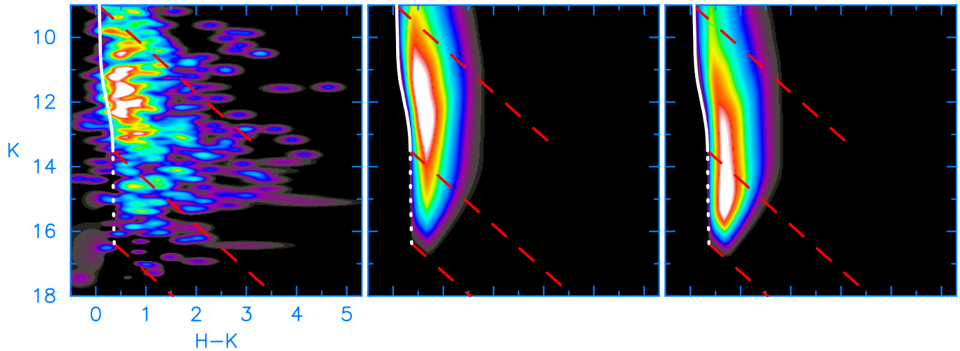
FIG. 12.—Simulations of the K-(H-K) diagram using the age distribution assumed from Fig. 8, the near-infrared excess distribution assumed from Fig. 9, and an extinction distribution that is uniform in the interval A_V = 0-5 mag. The middle panel shows the log-normal form of the Miller-Scalo mass function, while the right panel shows a shallow power law mass function [ N(\log M) \propto M^{-0.35} ]. Our data are shown in the left panel, which is the subtraction of the field star model in Fig. 7b from the observations in Fig. 7a. The models suggest that a falling mass function like that of Miller-Scalo better represents the peak in the observed ONC star counts than does an increasing mass function like the shallow power law. Although there appear to be some more highly extinguished stars in the data than in these models, broadening the A_V distribution in the models dilutes the peak; this suggests that the bulk of the ONC stars are found at relatively low extinction, A_V < 10 mag.
