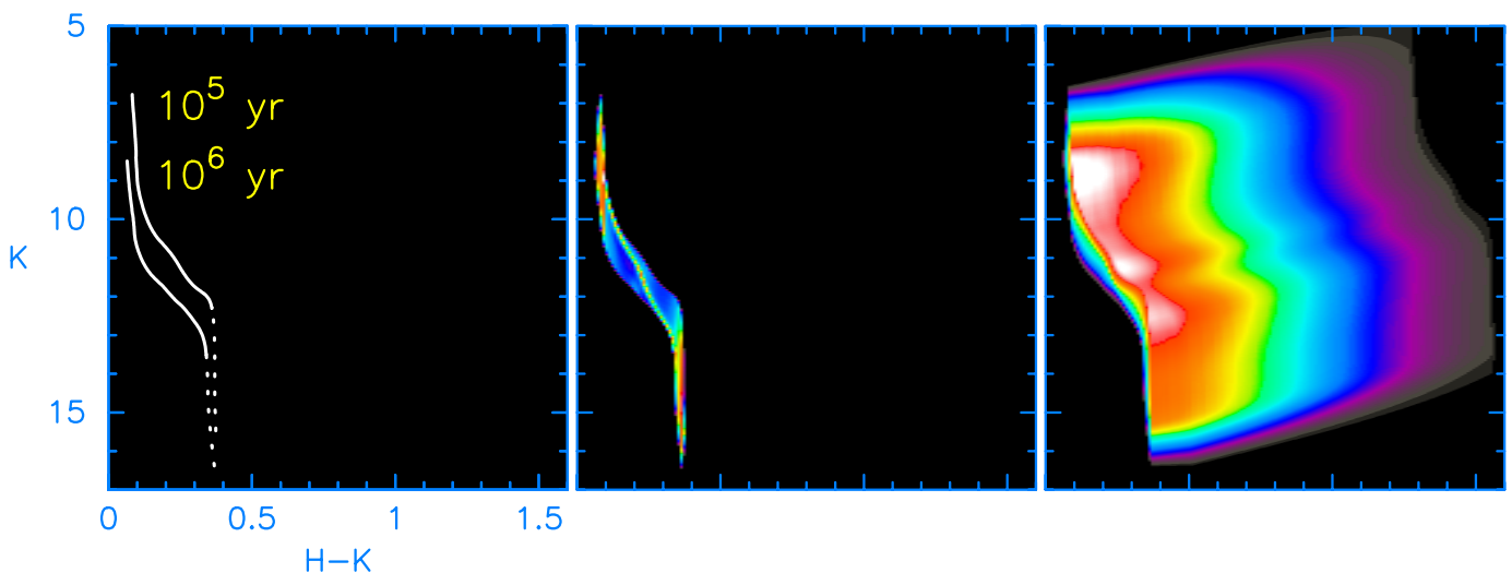
FIG. 11.—Model K-(H-K) diagrams for various assumptions about the age and near-infrared excess distributions. The mass function is log-uniform between 0.017 and 3.0 M_\odot . The left panel shows the K-(H-K) distribution of two single-aged populations at 10^5 and 10^6 years, with no near-infrared excess. The middle panel shows a population distributed log-uniform in age between 10^5 and 10^6 years, as we adopt for the ONC (see Fig. 8), and again with no near-infrared excess. The right panel shows the same log-uniform age distribution but now includes the near-infrared excess distribution adopted for the ONC (see Fig. 9).
