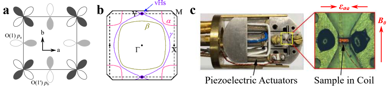
Figure S1: | RuO 2 plane, with d_{xy} - p hybridizing orbitals and experimental setup. a , Depiction of Ru d_{xy} - and hybridizing O p -orbitals at the Y-point, which dominate formation of the \gamma band. NMR shifts are measured at the O(1) and O(1') sites. b , Compressive a -axis stress shifts the \gamma band Fermi surface to the zone boundary at Y. c , Image of the strain device. The enlarged view highlights the Sr 2 RuO 4 single crystal mounted between piezoelectric actuators, with B_0 parallel to the b -axis and a -axis compressive stress, \epsilon_{aa} . The NMR coil covers the free part of \approx 1 mm length. density of states 16,17 . In Fig. S1c we show the sample mounted in the strain cell where \epsilon_{aa} \parallel a and B_0 \parallel b . The NMR coil was wrapped around the free part of the crystal, thus covering only the non-glued area that is subject to uniaxial stress. More information on strain-dependent NMR experiments on Sr 2 RuO 4 can be found in Ref. 17 .
