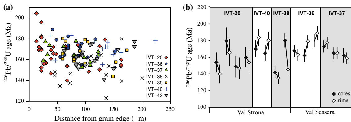
Fig. 6 a ^{207}\text{Pb} -corrected ^{206}\text{Pb}/^{238}\text{U} age versus distance from grain edge for IVZ rutile analyses. Error bars are omitted for clarity. Distance from the grain edge is taken as the shortest distance to the edge of the grain from the point of analysis, and is accurate
