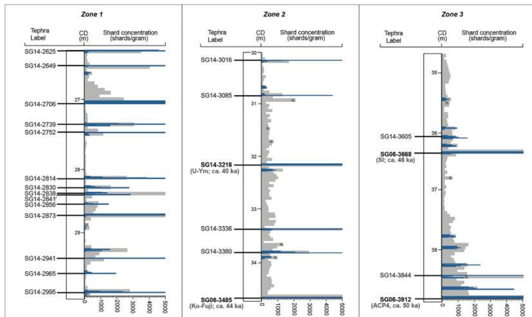
Figure 2. Glass shard concentrations (shards per gram of dry sediment; capped at 5,000) in the annually laminated sediments of the Lake Suigetsu SG14 core (50 to 30 ka). The tephratigraphy is divided into three zones (1–3) for illustrative purposes. Concentration of low-resolution (5 cm) samples are shown in gray, and high-resolution samples (1 cm) are overlain in blue. Tephra isochrons are labeled using their SG06/SG14 composite depth, with visible layers in bold. Peaks in shard concentrations that coincide with visible, high-energy event layers (EL) are not considered primary. SG06 visible tephra correlations and ages after Albert et al. (2018, 2019) and McLean et al. (2020).
