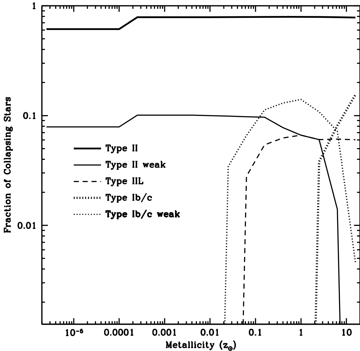
Fig. 1.— Single-star supernova rate as a fraction of total number of collapsing stars as a function of metallicity calculated using the stellar models from Heger et al.(2003). We consider 3 classes of type II supernovae: normal type II supernovae (Type II), Type II supernovae with weak supernova explosions (Type II weak), Type II supernovae that have lost most of their hydrogen envelope (Type IIL) and two classes of type Ib/c supernovae: normal Ib/c supernovae and weak Ib/c supernovae. If single stars dominate the Ib/c rate, these models predict only weak type Ib/c supernovae below solar metallicity.
