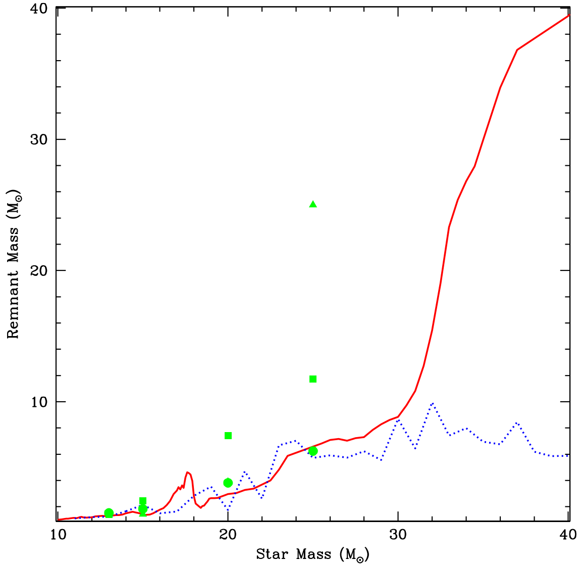
Fig. 4.— Remnant mass using the Fryer (2006) analysis versus initial star mass for both the Limongi & Chieffi (2006) and the Woosley et al. (2002) stellar progenitors. The lines are derived from the Woosley et al. (2002) progenitors: dotted line refers to solar metallicity, solid line refers to very low metallicity. The points are derived from the Limongi & Chieffi (2006) models: circle - solar, square - 0.2 solar, triangle - zero, metallicities. Around 20 M_{\odot} , the fate of the stars depend sensitively upon the stellar evolution code used. However, it is clear that around 20 M_{\odot} is roughly the dividing line between neutron star and black hole formation.
