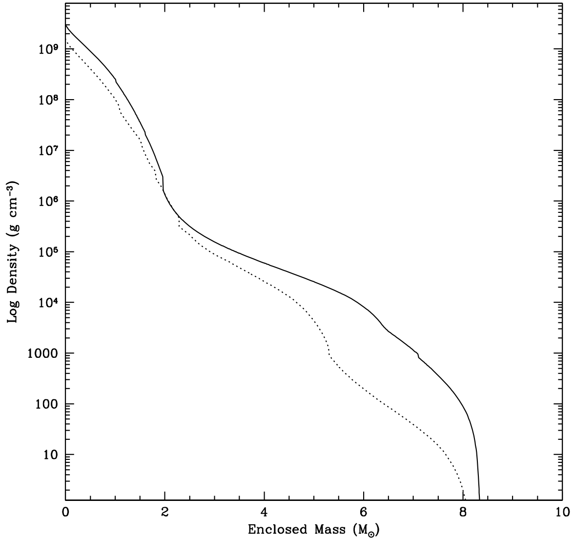
Fig. 5.— Density profiles of the Limongi & Chieffi (2006) and Woosley et al. (2002) 25 M_{\odot} stars at collapse. The differences in the inner 1 M_{\odot} can be explained by the fact that the models are at different stages in the collapse. A difference of a fraction of a second can cause the difference in densities in this inner region. But the differences beyond this inner core (beyond 2 M_{\odot} ) can only be explained by uncertainties in the stellar evolution models.
