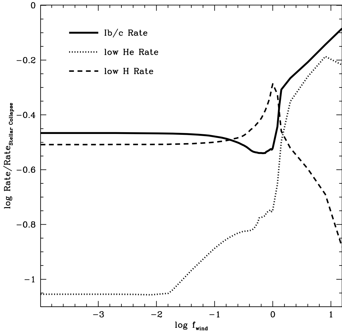
Fig. 2.— Binary-star supernova rate as a function of the mass loss parameter (see Fryer et al. 1998 for details). We consider three types of supernovae: all type Ib/c supernovae, type Ib/c supernovae that have lost more than 1 M_{\odot} of helium (not necessarily type Ic supernovae, but on their way to becoming Ic supernovae), and type II supernovae that have lost 2/3 of their hydrogen (peculiar type II or type III supernovae) but still retain some hydrogen envelope to be type II supernovae. As the mass-loss parameter increases, the rate of Ib/c and low-helium supernovae increases while the rate of low hydrogen (and all type II supernovae for that matter) decreases. This mass-loss parameter can be seen as a parameter for the metallicity. Although the rate of Ib/c supernovae is higher at higher mass-loss rates (higher metallicities), it drops less than a factor of 5 when varying the mass-loss parameter from very high mass-loss to essentially no mass-loss rates.
