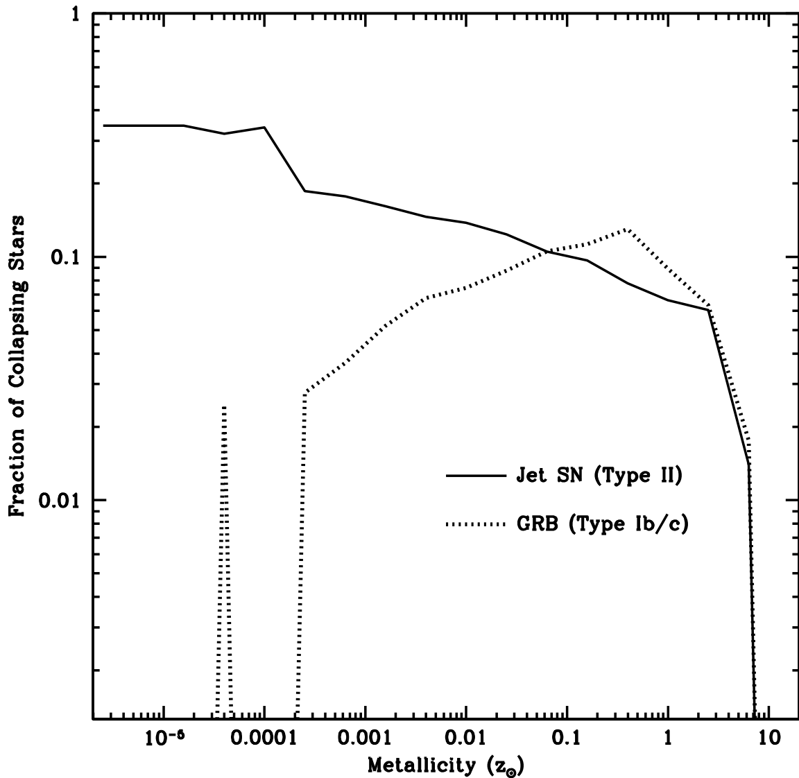
Fig. 6.— GRB rate as a function of collapsing stars for single stars as a function of metallicity using the Heger et al.(2003) models. The solid line shows those possible hypernovae with hydrogen envelopes (termed “jet” supernovae by Heger et al. 2003). The dotted line shows systems that lose their hydrogen envelopes and hence could be GRB progenitors. These numbers must be multiplied by a factor indicating what fraction of these stars actually retain enough angular momentum to make black hole accretion disks (could be 0). To make single models work, we must somehow explain why we don’t observe jet supernovae (currently a matter of debate in stellar evolution theory).
