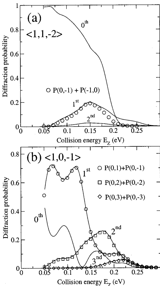
FIG. 6. Shown are the probabilities for diffraction into the zeroth to third diffraction order, for incidence along the \langle 11\bar{2} \rangle (a) and \langle 10\bar{1} \rangle (b) direction. The initial parallel energy E_{\parallel} = 0.48 eV. Also, for the \langle 10\bar{1} \rangle incidence direction, the summed probability is plotted for diffraction into the diffraction channels (0, m) and (0, -m) , that belong to the m th diffraction order and correspond to out-of-plane diffraction. For the \langle 11\bar{2} \rangle incidence direction, we also show the sum of the probabilities for diffraction into the (0, -1) and (-1, 0) states.
