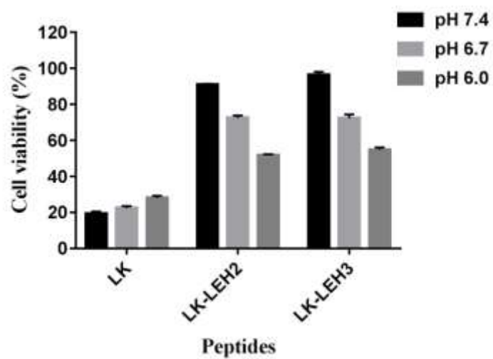
Figure S1 pH-dependent antitumor activity of LK-LEH2 and LK-LEH3 at 20 \mu M to HeLa cells at different pH values (pH 7.4, 6.7 and 6.0). Data are representative of triplicate experiments.
