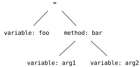
Fig. 2. An example of an assignment in AST form.
