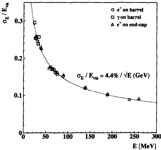
Fig. 10. Energy resolution for photons and positrons vs kinetic energy.
