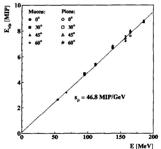
Fig. 12. Energy response for muons and pions vs kinetic energy.
