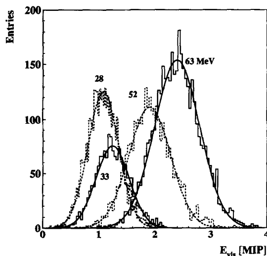
Fig. 5. Energy spectra for photons.
