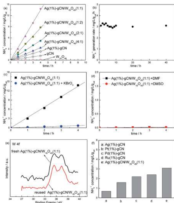
Fig. 6 Photocatalytic NH_4^+ production ability of as-prepared catalysts (a), N_2 photofixation stability of Ag(1%)-gCN/ W_{18}O_{49}(1:1) (b), NH_4^+ production ability of Ag(1%)-gCN/ W_{18}O_{49}(1:1) using KBrO_3 as the electron scavenger (c) or in aprotic solvents DMF and DMSO (d), XPS results of fresh and reused Ag(1%)-gCN/ W_{18}O_{49}(1:1) in the region of W 4f (e) and N_2 photofixation ability of Ag(1%)-gCN, Ag(1%)-gCN/ W_{18}O_{49}(1:1) , Pt(1%)-gCN, Pd(1%)-gCN and Ru(1%)-gCN under simulated solar light (f).
