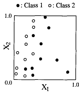
Fig. 16. Classification problem.
