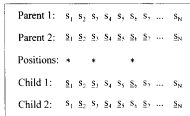
Fig. 10. Illustration of the crossover operation. Bit values at the marked positions are interchanged in the two parents to form two children.
